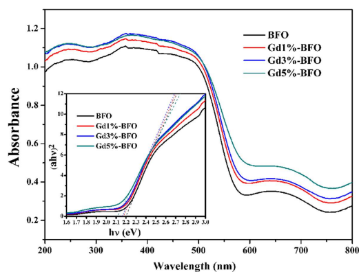
Figure 5. UV-vis diffuse reflectance spectra of as-prepared pure BFO and Gd-doped BFO samples. Insets are the plots to determine the band gaps for the each sample.
