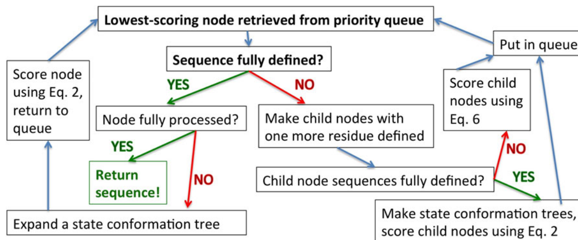
FIG. 3. COMETS is a sequence of node-processing operations.
