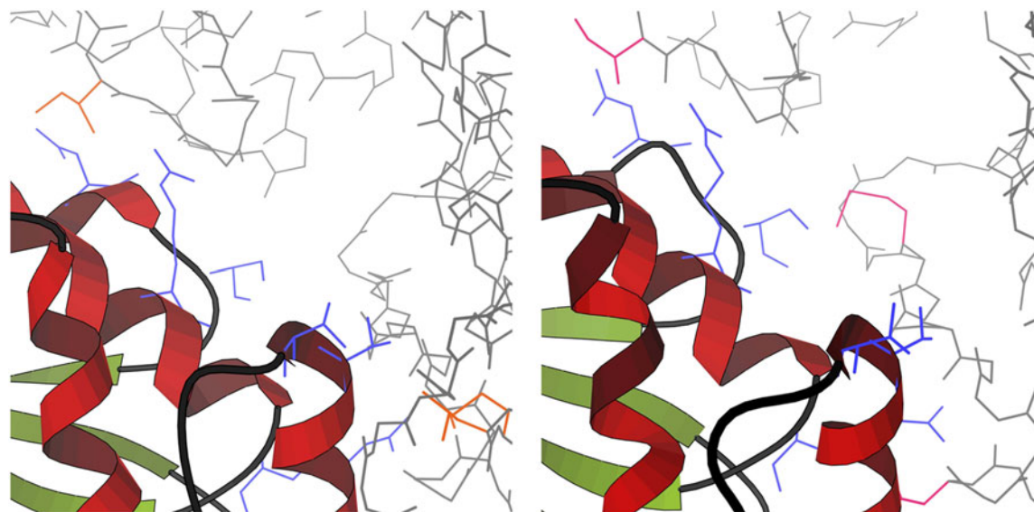
FIG. 1. Flexible and mutable residues in a design for specificity. The apoptotic regulator CED4 forms two different dimers, one to block apoptosis ( left ; PDB id 2a5y [Yan et al., 2005]) and one to induce it ( right ; PDB id 3lqr [Qi et al., 2010]). We want to design for specificity (to block apoptosis), so we allow mutations to some residues in the binding site (blue). To accurately model the conformational changes induced by the mutations, we also model as flexible the residues on the opposite side of each interface that interact with the mutable residues (orange, pink). Analysis of this calculation and others is described in section 3.
