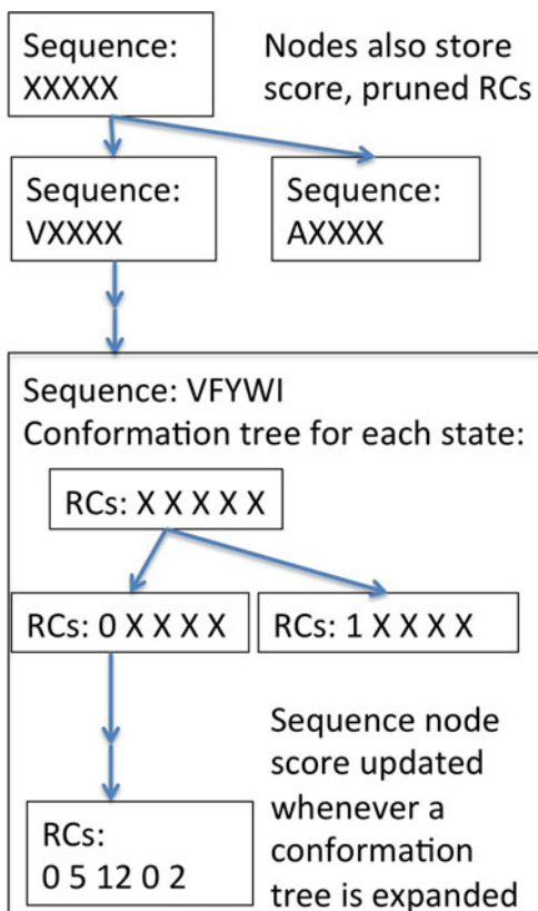
FIG. 2. Expansion steps during node processing generate nodes with partially (e.g., VXXXX or AXXXX) and then fully (e.g., VFYWI) defined sequences. Once a node has a fully defined sequence, conformational trees are built for it for all states. Then conformational tree expansions lead to fully processed nodes. X, unassigned amino acid or RC; V, Val; A, Ala; F, Phe; Y, Tyr; W, Trp; I, Ile.
