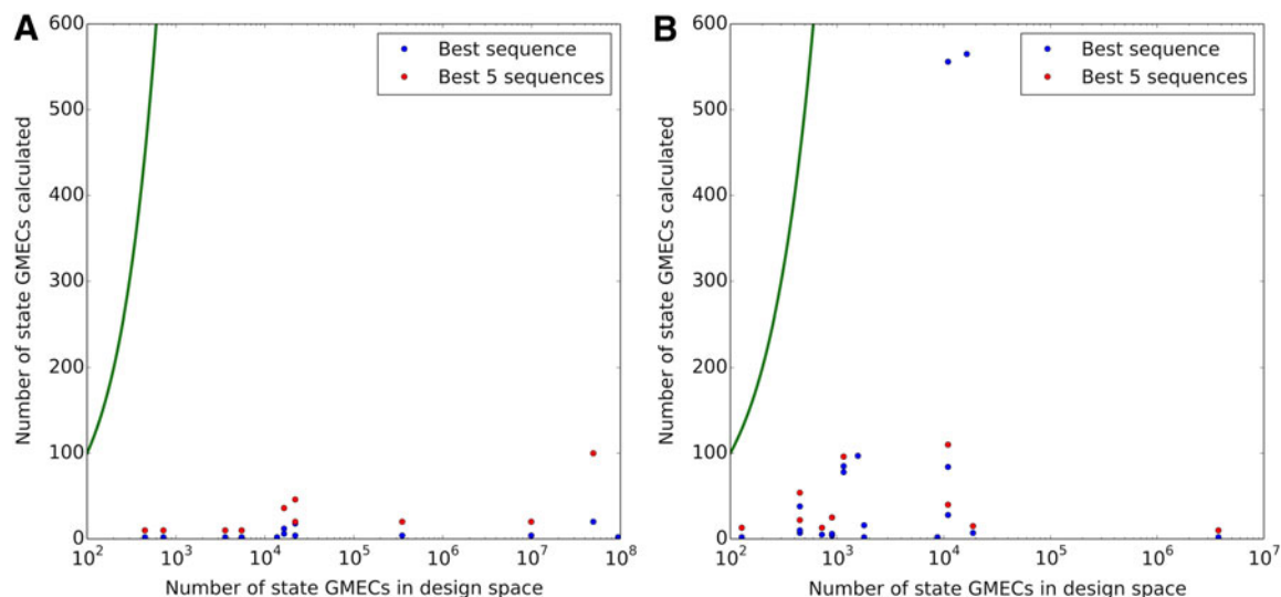
FIG. 4. Number g of state GMECs calculated in COMETS runs with (A) rigid or (B) continuous flexibility, compared to the number sN of state GMECs in the entire design space ( sN is the number of sequences in the design space times the number of states). Results are shown both for calculation of the best sequence and for enumeration of the best five, when possible under the design constraints. Exhaustive search would have to calculate all state GMECs (green curve).
