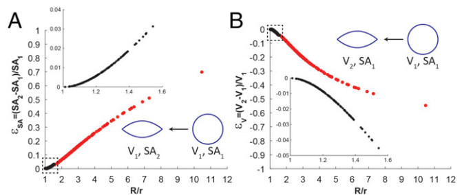
Fig. 3. Fractional changes in surface area and volume calculated to accompany LC-induced GUV shape transformations. (A) Fractional GUV surface area expansion ( \epsilon_{SA} ) calculated for an LC-induced GUV shape transformation at constant internal GUV volume. (B) Fractional change in GUV internal volume ( \epsilon_V ) calculated for an LC-induced GUV shape transformation at constant GUV membrane surface area. Data in red denote GUVs with cusp angles \alpha < 130^\circ , and data in black denote GUVs with cusp angles \alpha > 130^\circ .
