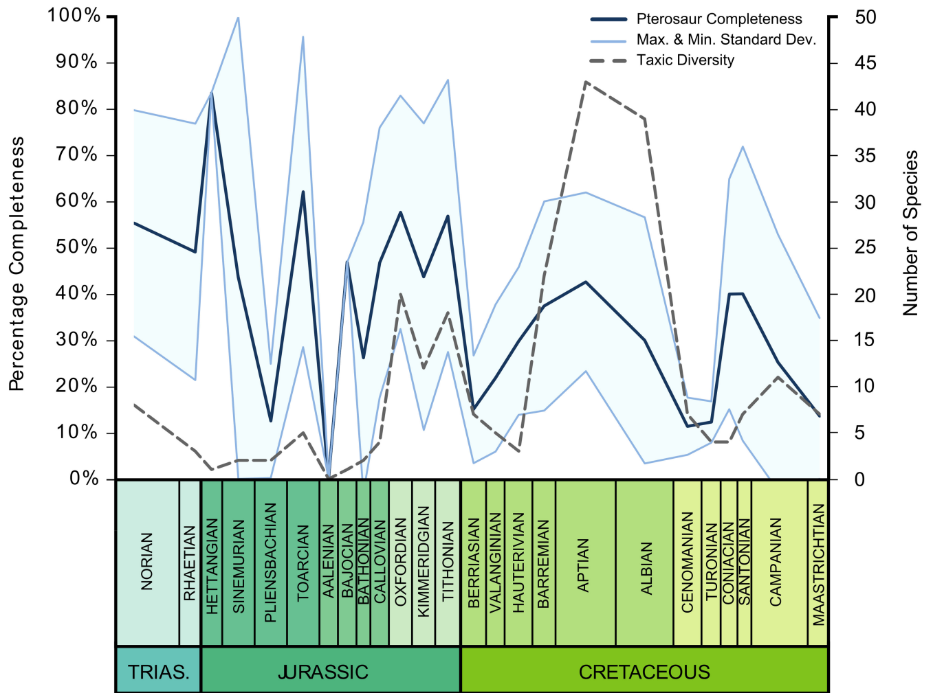
Figure 1. Completeness and taxic diversity of pterosaurs throughout the Mesozoic. Light blue areas surrounding Character Completeness Metric represent one standard deviation around the mean.
