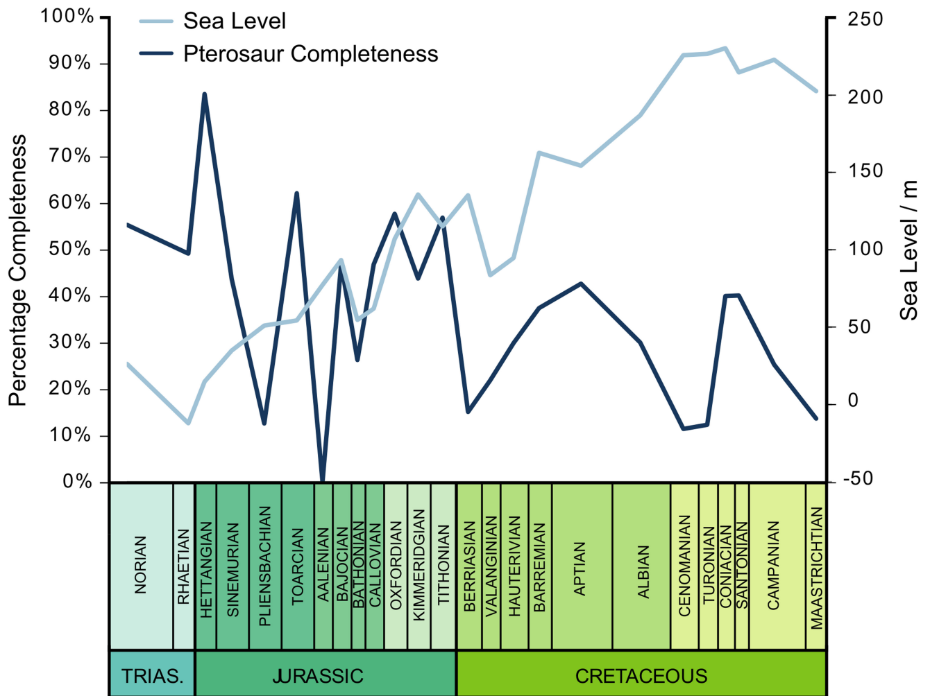
Figure 7. Comparison between global sea level (Butler et al. 2013, after Haq et al. 1987) and pterosaur completeness for the Mesozoic.
