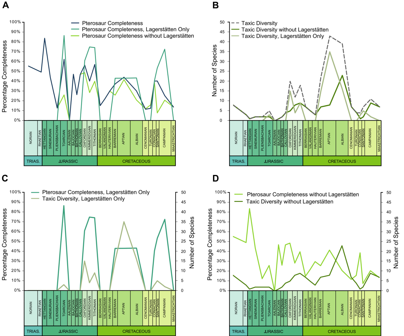
Figure 4. Plots of Lagerstätten groupings plotted throughout the Mesozoic. A , Overall pterosaur completeness compared with subgrouping of Lagerstätten only and Lagerstätten removed completeness. B , Overall pterosaur diversity compared with subgrouping of Lagerstätten only and Lagerstätten removed diversity. C , Lagerstätten only completeness and diversity. D , Lagerstätten removed completeness and diversity.
