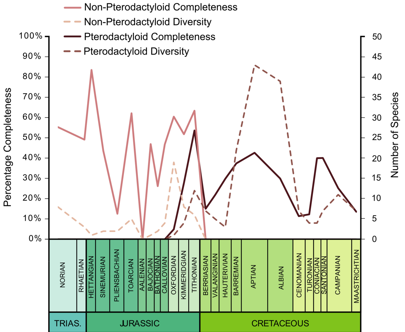
Figure 6. Plots showing completeness and diversity in subgrouping of Pterodactyloidea and non-Pterodactyloidea throughout the Mesozoic.
