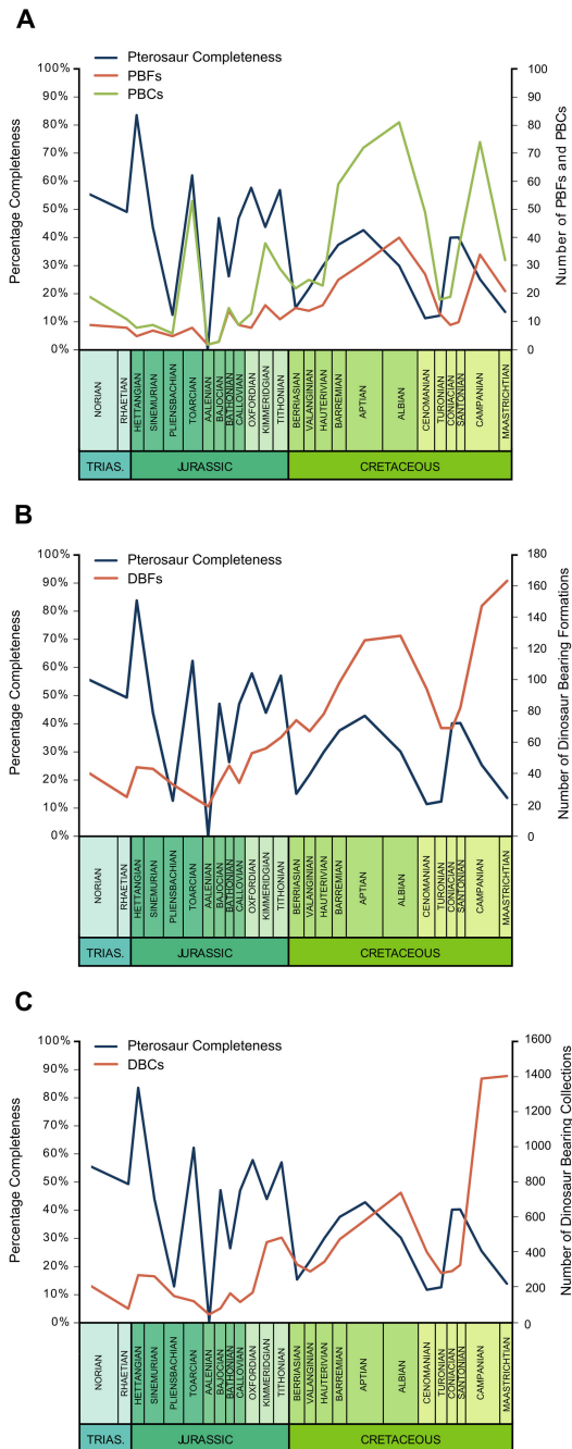
Figure 2. Sampling proxies plotted throughout the Mesozoic. A , Pterosaur completeness, Pterosaur Bearing Formations and Pterosaur Bearing Collections. B , Pterosaur completeness and Dinosaur Bearing Formations. C , Pterosaur completeness and Dinosaur Bearing Collections.
