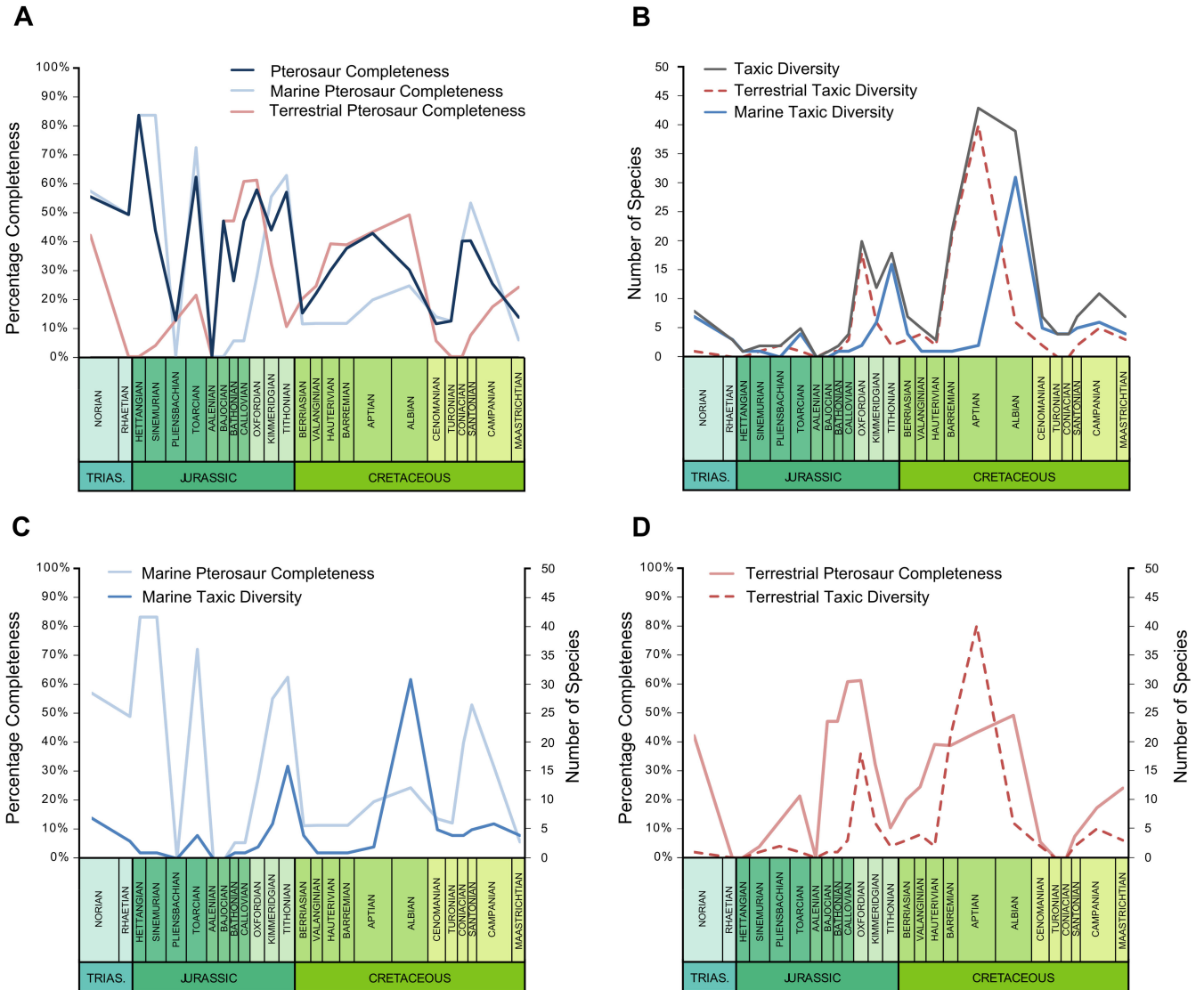
Figure 5. Plots of pterosaurs found within marine and terrestrial environments for all stages of the Mesozoic. A , Overall pterosaur completeness compared with subgrouping of marine and terrestrial completeness. B , Overall pterosaur diversity compared with subgrouping of marine and terrestrial diversity. C , Marine completeness and diversity. D , Terrestrial completeness and diversity.
