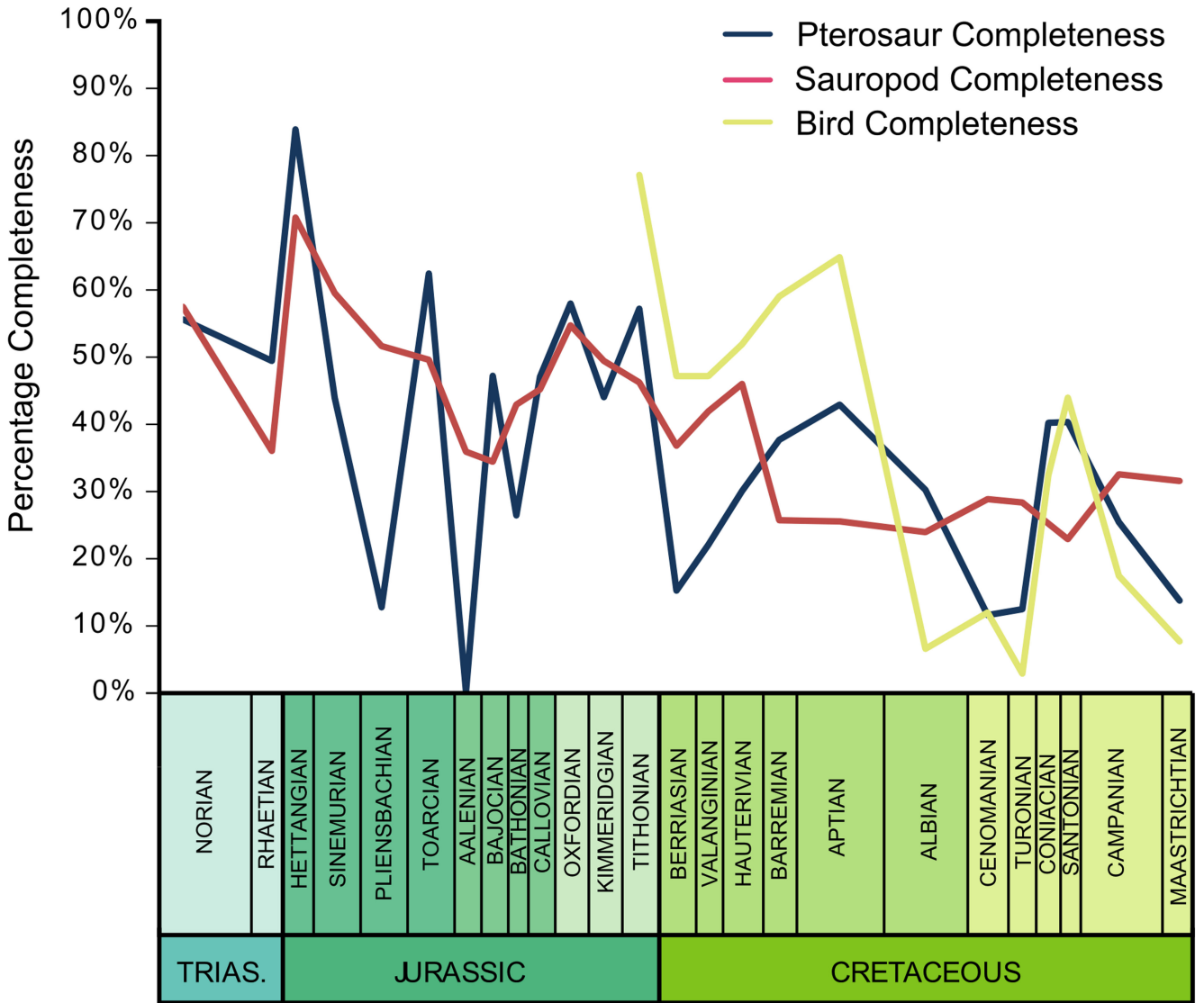
Figure 3. Pterosaur, bird and sauropodomorph completeness plotted throughout the Mesozoic. Bird completeness is not available prior to the Tithonian.
