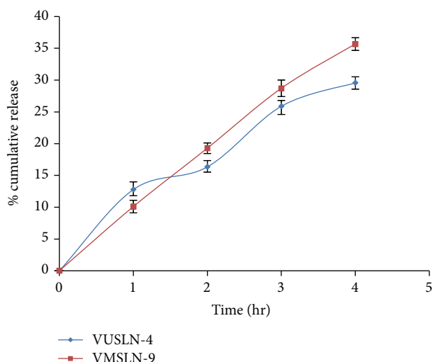
FIGURE 6: Transcorneal permeation profile of voriconazole from optimized SLN formulation through excised goat cornea.
