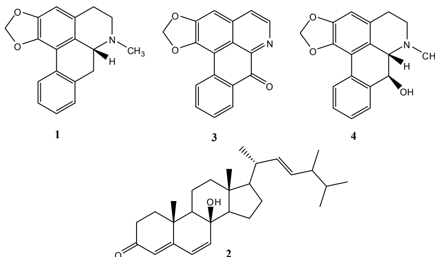
Figure 1. Structure of compounds 1–4.
