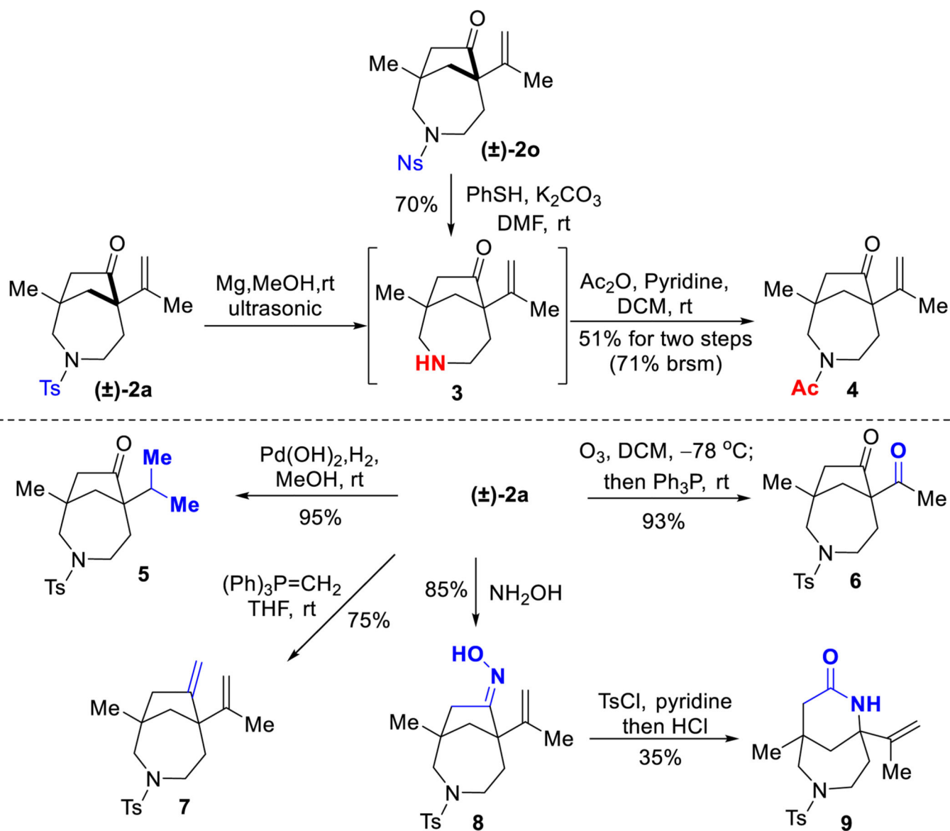
Scheme 3. Synthetic Applications
