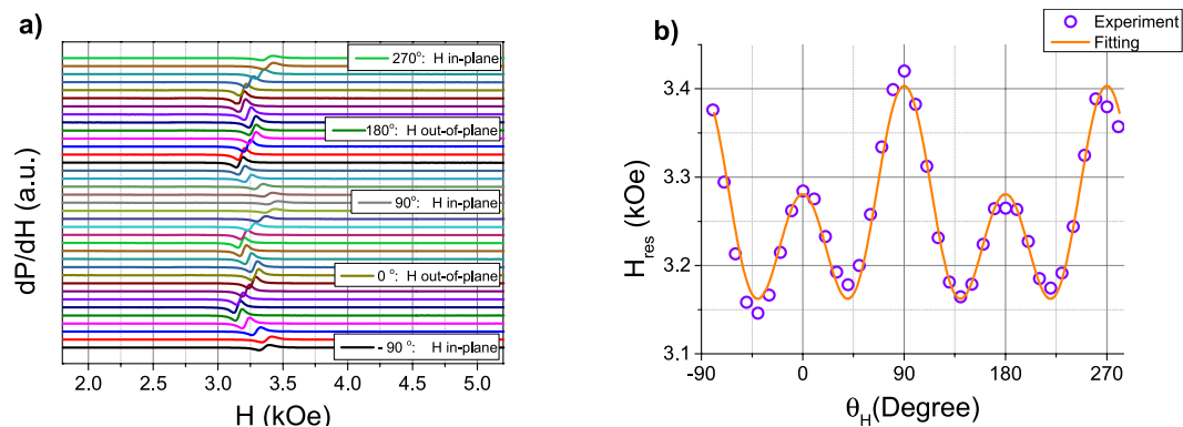
Figure 9. Angular dependent out-of-plane FMR measurements on the sample with t = 16.9 Å. (a) 10-degree step FMR spectra with magnetic field angle counted from the film normal. (b) extracted angular dependence of FMR resonance field and respective fitting using Smit-Beljers formalism.
