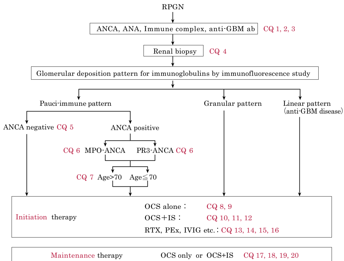
Fig. 2 Differential diagnosis of RPGN and treatment options. The algorithm for diagnosis and treatment with corresponding CQs are shown in this figure. OCS oral corticosteroid, IS immunosuppressant, PEx plasma exchange, RTX rituximab, IVIG intravenous immunoglobulin
