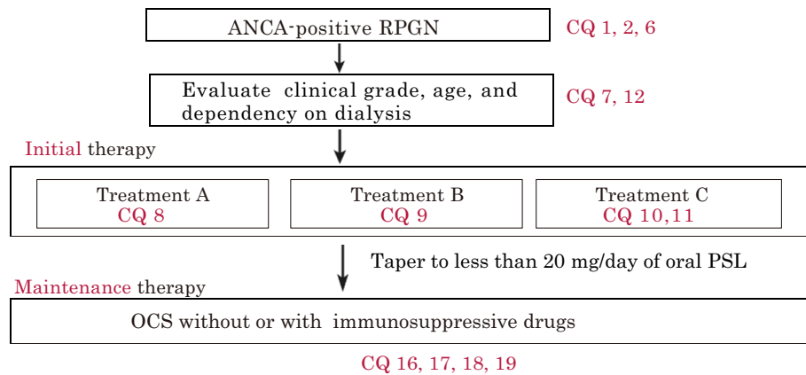
Fig. 1 Treatment algorithm for ANCA-positive RPGN and CQs (changed from reference: the RPGN clinical practice guide 2011 by the Progressive Renal Disease Research, from the Ministry of Health, Labour and Welfare of Japan). Asterisk For older patients over 70 years, lower-grade treatment may be considered including the regimen without pulse methylprednisolone. Asterisk At the
