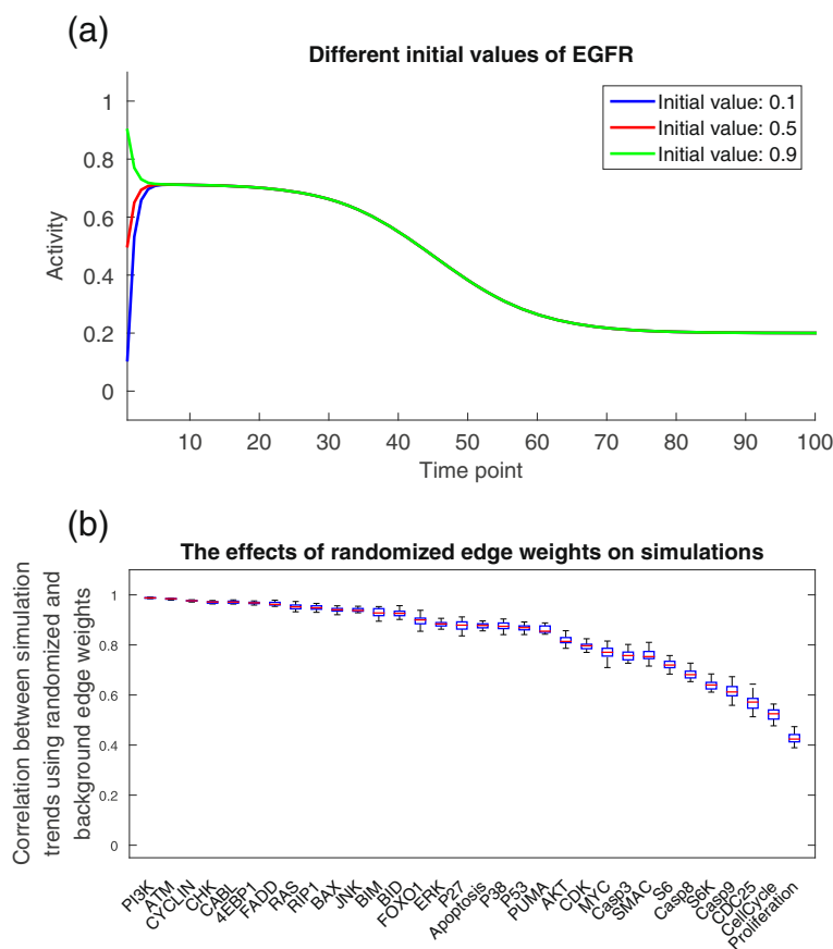
Fig. 4 a The influence of different initial values on simulations. The initial value does not change the main trend of the state transition and the level of the stable state. b The influence of different edge weights to simulations. Each of the 32 signals shows a small range of the correlations between the simulated and the background trends, indicating that the proposed model is robust to different edge weights
