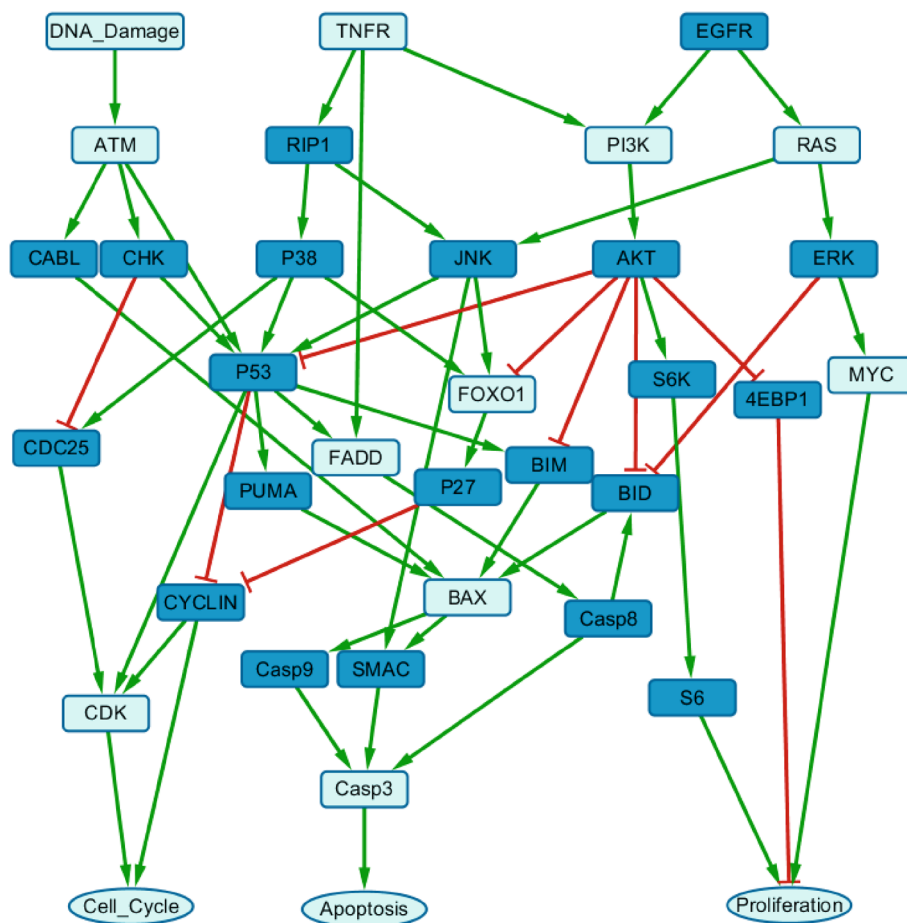
Fig. 2 Signaling pathways constructed based on the dataset in [18]. Round rectangles and ellipses represent signaling proteins (or stimuli) and cell fates, respectively. The signals that have measurements in the dataset [18] are represented by dark blue nodes. Each activation interaction is denoted as a green edge with an arrow head and each inhibition interaction is represented by a red edge with a flat-head
