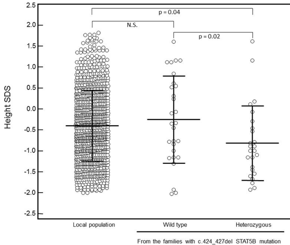
Figure 1. Comparison of height SDS distribution among adult heterozygous carriers of STAT5B c.424_427del mutation (n = 25), their non-carrier relatives (n = 28) and a population sample from the same region in the south of Brazil (n=1,099).
