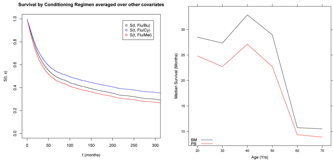
Figure 6. Left Panel: Partial Dependence Survival functions for 3 different conditioning regimens (Flu=Fludarabine, Bu=Busulfan, Cy=Cyclophosphamide, Mel=Melphalan); Right Panel: Median survival by age and graft type (BM= Bone Marrow, PB=Peripheral Blood)
