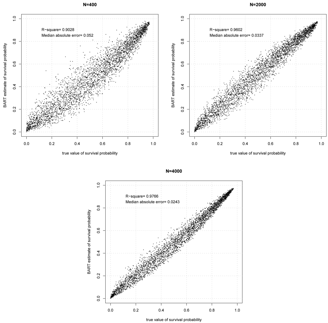
Figure 5. Plots of BART estimated survival probabilities vs true probabilities for the model with highly nonlinear relationship with covariates.
