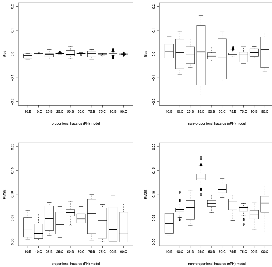
Figure 4. Box plots of bias and RMSE for all 512 configurations averaged over 400 simulated data sets, for PH (left) and nPH (right) models. Horizontal axes markings indicate the percentile of the overall survival at which probabilities were estimated, followed by the estimation method: B for BART, C for Cox regression.
