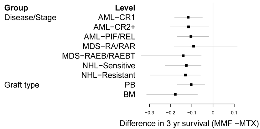
Figure 7. Forest plot of the difference in 3 year survival between MMF(Mycophenolate Mofitol) and MTX(Methotrexate), separately by disease/stage (AML=Acute Myelogenous Leukemia, MDS=Myelodysplastic Syndrome, NHL=Non-Hodgkin's Lymphoma, CR=Complete Remission, PIF=Primary Induction Failure, REL=Relapse, RA=Refractory Anemia, RAR=RA with Ringed Sideroblasts, RAEB=RA with Excess Blasts, RAEBT=RAEB in Transmission) and graft type (PB=Peripheral Blood, BM=Bone Marrow). Negative values indicate MMF has worse outcomes.
