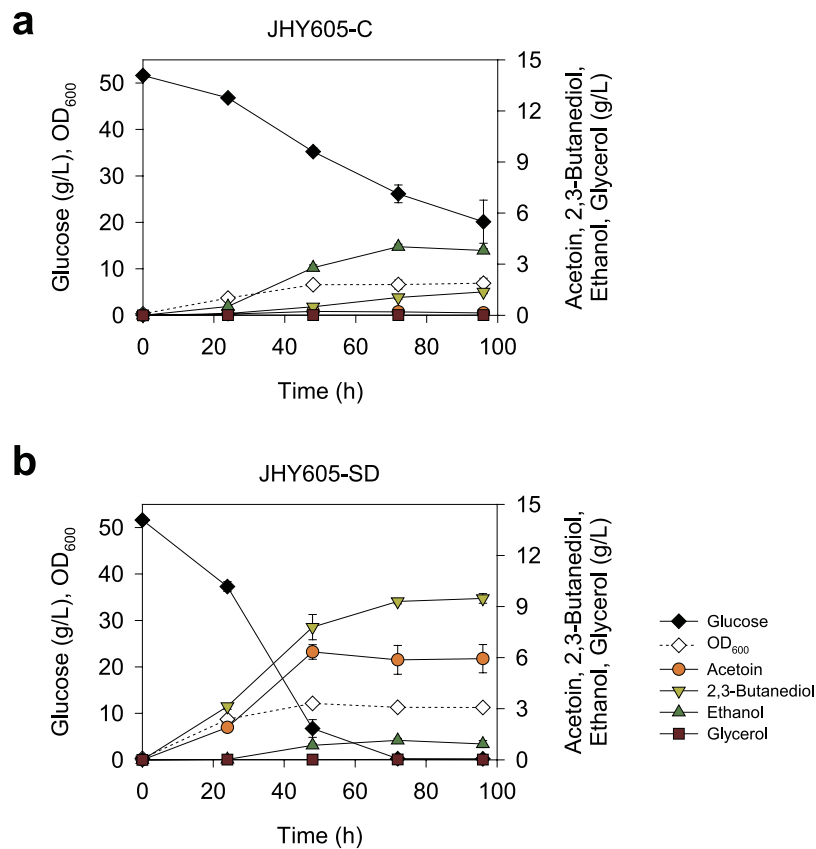
Figure 2. Acetoin production by introducing acetoin biosynthetic pathway. Strain JHY605 ( adh1-5Δgpd1Δgpd2Δ ) harboring empty p413GPD plasmid (JHY605-C) (a) or p413-SD (JHY605-SD) (b) was grown in 10 mL SC-His media containing 50 g/L glucose in a 100 mL flask. Error bars indicate standard deviations of three independent experiments.
