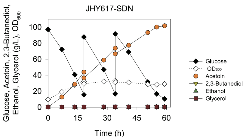
Figure 4. Fed-batch fermentation of JHY617-SDN for acetoin production. Strain JHY617-SDN was cultivated in YPD medium containing 100 g/L glucose with initial OD 600 of 9.5. Glucose was intermittently added into culture medium using the feeding solution (800 g/L glucose) before glucose was completely consumed.
