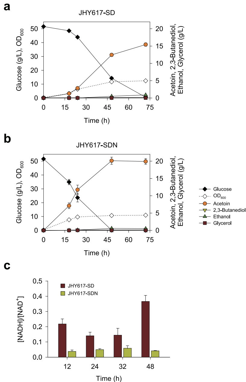
Figure 3. Improvement of acetoin production by deleting BDH1 and by expressing NADH oxidase (NoxE). Strain JHY617 ( adh1-5Δgpd1Δgpd2Δbdh1Δ ) harboring p413-SD (JHY617-SD) (a) or p413-SDN (JHY617-SDN) (b) was grown in 10 mL SC-His containing 50 g/L glucose in a 100 mL flask. (c) NADH/NAD + ratios in JHY617-SD and JHY617-SDN. Error bars indicate standard deviations of three independent experiments.
