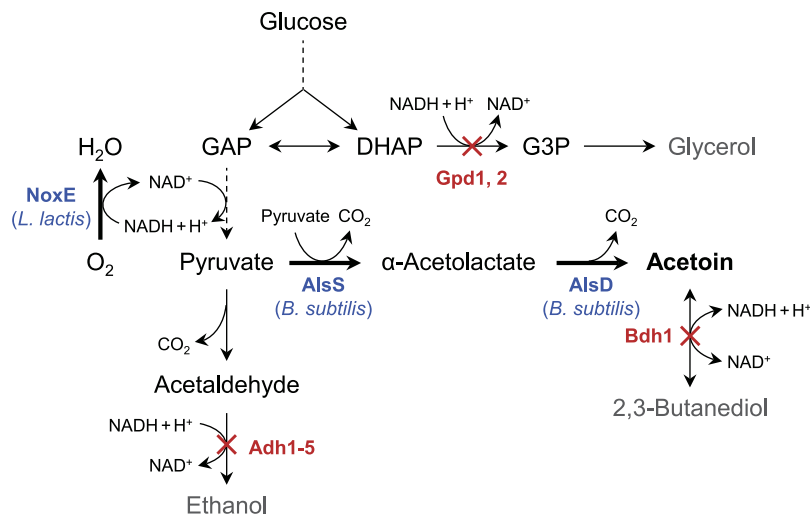
Figure 1. Metabolic pathway for acetoin production used in this study. Two molecules of pyruvate are converted to one molecule of acetoin by \alpha -acetolactate synthase (AlsS) and \alpha -acetolactate decarboxylase (AlsD). Acetoin can be further reduced to 2,3-butanediol by 2,3-butanediol dehydrogenase (Bdh1). The water-forming NADH oxidase (NoxE) catalyzes the oxidation of NADH to NAD + using oxygen as an electron acceptor. Dashed arrows indicate multiple enzymatic steps. The crosses represent blockage of the pathway by deleting the corresponding genes. DHAP, dihydroxyacetone phosphate; G3P, glycerol-3-phosphate; GAP, glyceraldehyde-3-phosphate.
