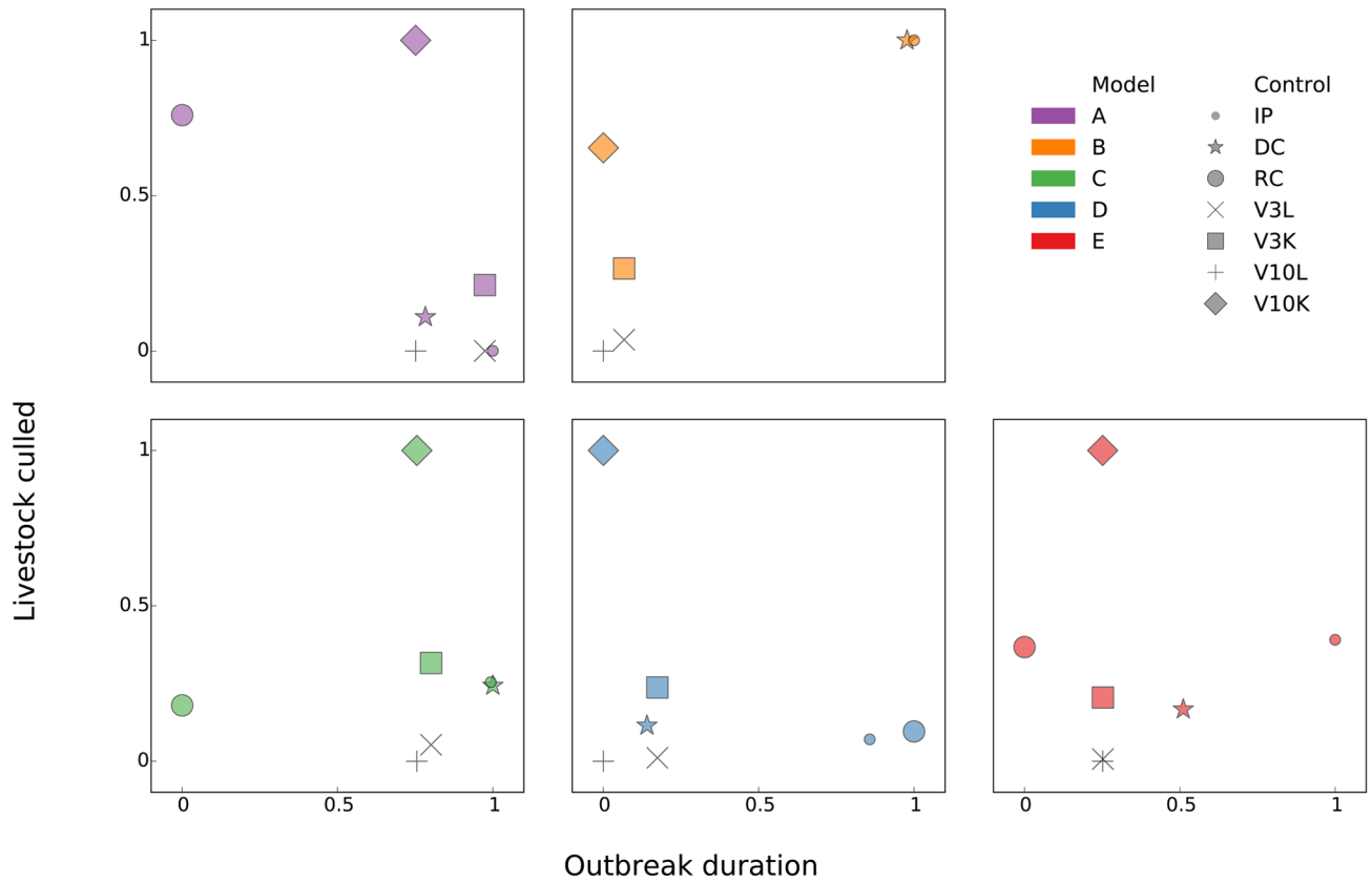
Figure 4. Performance of control strategies under both mean outbreak duration and mean number of livestock culled across five simulation models of FMD spread. Mean values from simulation output under each model and under each measure of success (outbreak duration and livestock culled) have been scaled so that the worst control strategy has a score of 1 and the best a score of 0 within each model.
