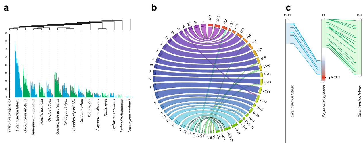
Fig. 5 Comparative genomics analysis. a The percentage of P. oxygeneios ddRAD sequences per linkage group that showed homology with sequences from other fish genomes, listed on the x-axis; * P. marinus : outgroup. The phylogenetic tree provided above the graph is based on recent classifications [30–32]. b Schematic of homology between proposed linkage groups (1–35) and published D. labrax linkage groups. Only blocks of 2 markers or more are illustrated; The complete comparative analysis for all species is summarised in Additional file 11: Table S7. c Graphic identifying syntenic regions between P. oxygeneios LG 14 and D. labrax linkage groups
