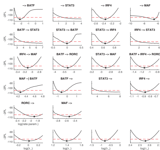
Fig. 5. Parameter profile likelihood for the parameters of the inferred Th17 core network LEM model. The first five rows show the estimated profile likelihoods for the rate parameters and the bottom row shows the estimated profile likelihoods for the parameters of the latent process. The dashed red line shows the 95% confidence threshold and the asterisk shows the maximum likelihood estimate of the parameter when a unique value is available
