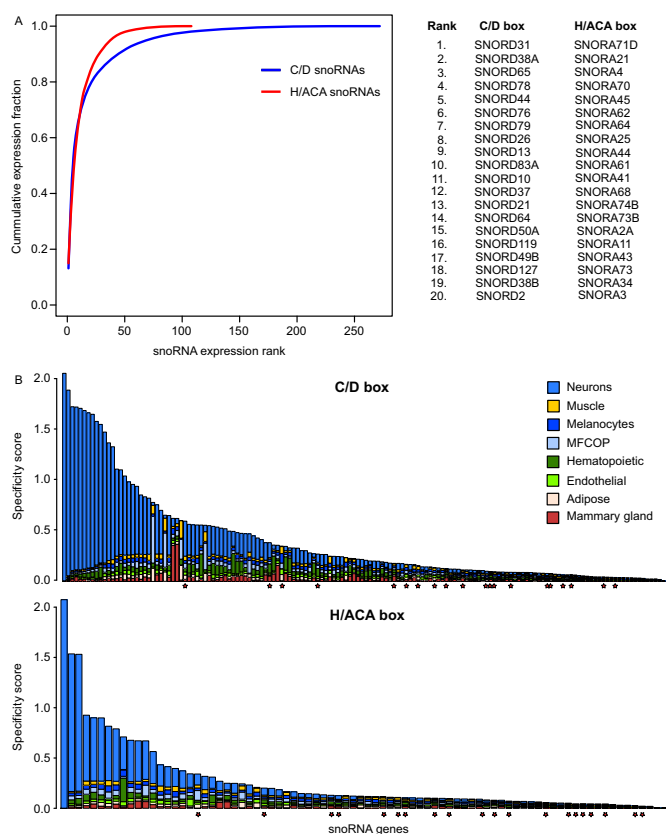
Figure 6. Expression profiling of snoRNA genes in ENCODE sRNA-seq data. (A) The pool of human snoRNA genes is dominated by a few abundantly expressed snoRNA genes. (B) Evaluation of tissue specific expression of snoRNA genes. The top panel shows values for C/D box snoRNAs, while the bottom panel does for H/ACA box snoRNAs. The higher the specificity score is the more biased is the expression to a specific tissue or cell type. MFOCP is an acronym for melanocytes, fibroblasts, osteoblasts, chondrocytes and placental tissue. The red stars mark the 20 most highly expressed C/D box (upper panel) and H/ACA box (lower panel) snoRNAs in the entire data set (further details in Supplementary Figure S2).
