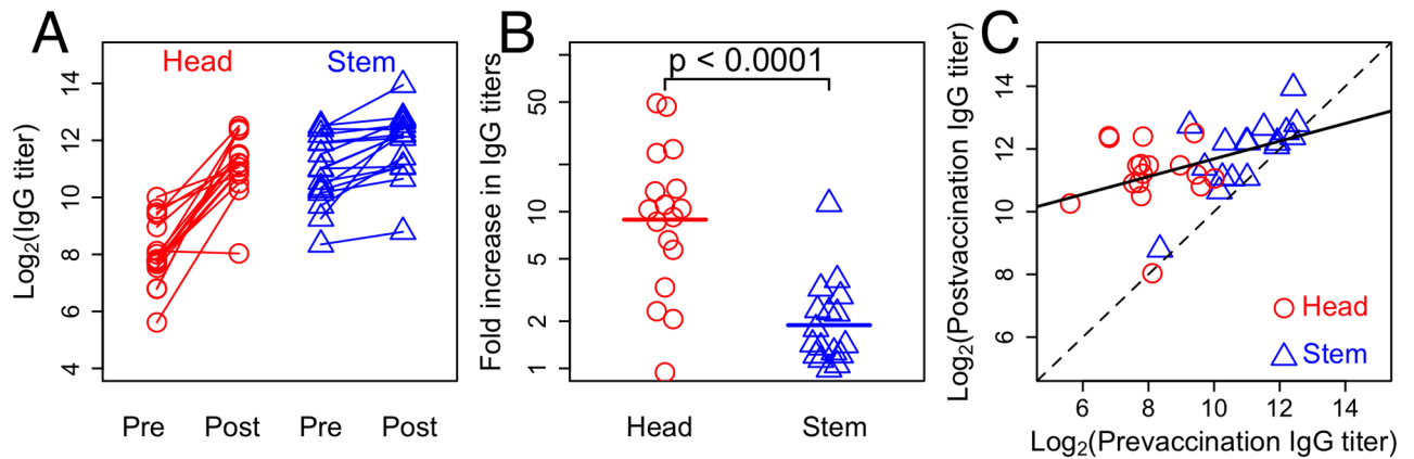
Fig 1. Boosting of antibodies to the head and stem epitopes of HA following vaccination with inactivated H5N1. Panel A shows IgG titers against HA head (red) and stem (blue) epitopes measured prevaccination and 30 days post-vaccination. Panel B shows the fold-increase in IgG antibody titers against HA head (red) and stem (blue) epitopes calculated from the data in panel A. Panel C shows the relationship between the pre- and post-vaccination antibody titers. In the absence of boosting, we expect the data to fall on the dashed line (slope = 1). If the degree of boosting is independent of the initial titer, boosting would result in the data falling on a line parallel to (and above) the dashed line. The solid line, representing the best fit line, has slope less than one (least squares; slope = 0.28; 95% CI = [0.090;0.476]), indicating that there is less boosting when initial antibody titers are high. Data are from [20].
