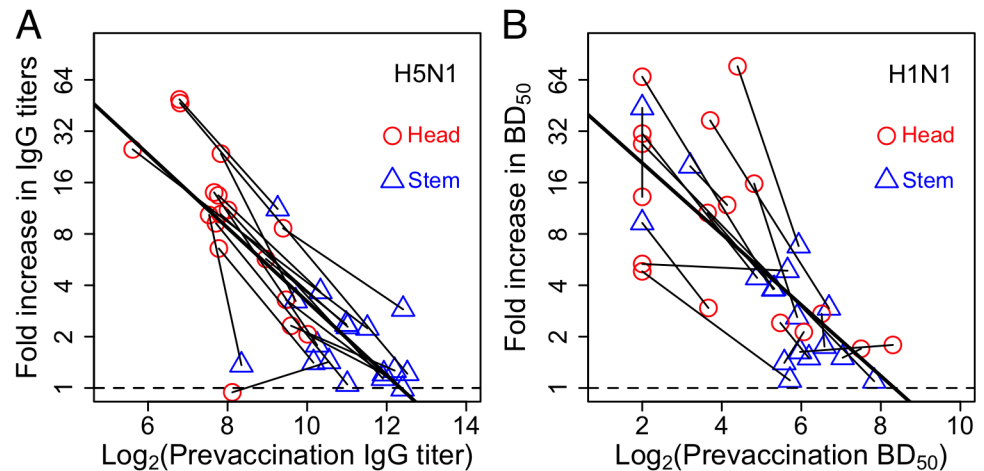
Fig 6. Analysis for how the fold increase in antibodies to the head and stem of HA depend on their pre-immune levels in individuals. We plot lines obtained by joining the data for head and stem for individuals vaccinated with H5N1 (Panel A) and H1N1 (Panel B) (see Tables C and D in S1 Text ). We find the slope of these lines is not significantly different from an average line using all the data (thick line). This result consistent with the EMM model, but inconsistent with the ACM and FIM models which predict the slopes of the individual lines should be zero. Also see corresponding Table 2 .
