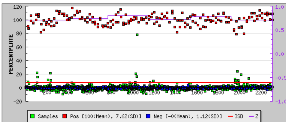
Fig. 6. HTS data with IEDDA-based cat-ELCCA.
