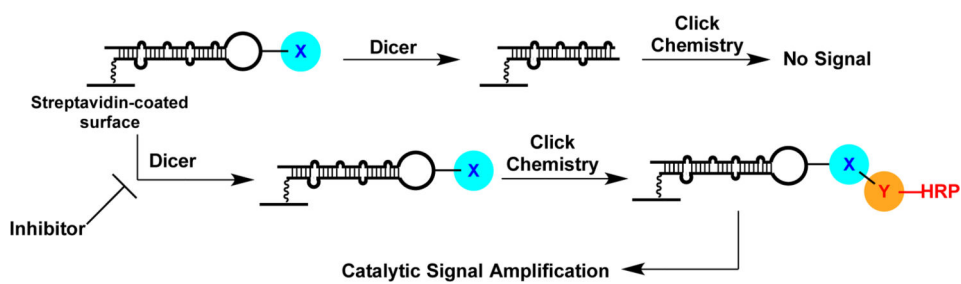
Fig. 2. cat-ELCCA for Dicer-mediated pre-miRNA maturation.
