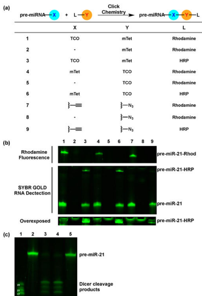
Fig. 3. Comparison of in-solution click reactions and Dicer cleavage. (a) General scheme and table of click reactions. - = no pre-miRNA. (b) pre-miRNA IEDDA products detected via fluorescence gel. Click reactions were performed with 2.0 equiv. of L-Y for 2 h at 25 °C. Top = Detection of rhodamine-pre-miRNA conjugate. Rhodamine fluorescence was first detected, followed by addition of SYBR GOLD for 5 min and RNA detection on the same gel. Middle = Detection of HRP-pre-miRNA conjugate using SYBR GOLD. Bottom = Overexposure and zoom of the band representing the HRP-pre-miRNA conjugate. (c) pre-miRNA maturation catalyzed by Dicer. Lane 1 = miRNA ladder; Lane 2 = pre-miRNA-TCO; Lane 3 = pre-miRNA-TCO + Dicer; Lane 4 = pre-miRNA-mTet + Dicer; Lane 5 = pre-miRNA-mTet.
