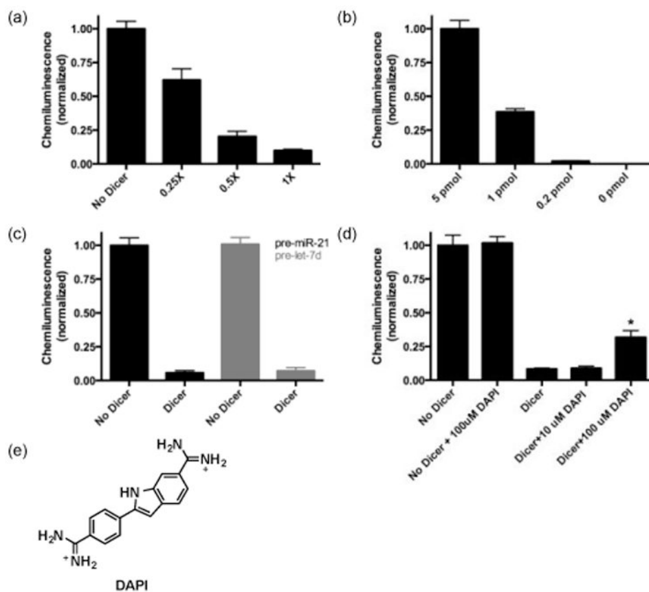
Fig. 5. Characterization of IEDDA-based cat-ELCCA. Dependence on: (a) Dicer; (b) Immobilized pre-miRNA; (c) pre-miRNA substrate; (d) DAPI binding. Significance was determined using a two-tailed, unpaired t-test. p -values of 0.6 and <0.0001 were calculated for 10 μM and 100 μM DAPI, respectively. (e) DAPI structure.
