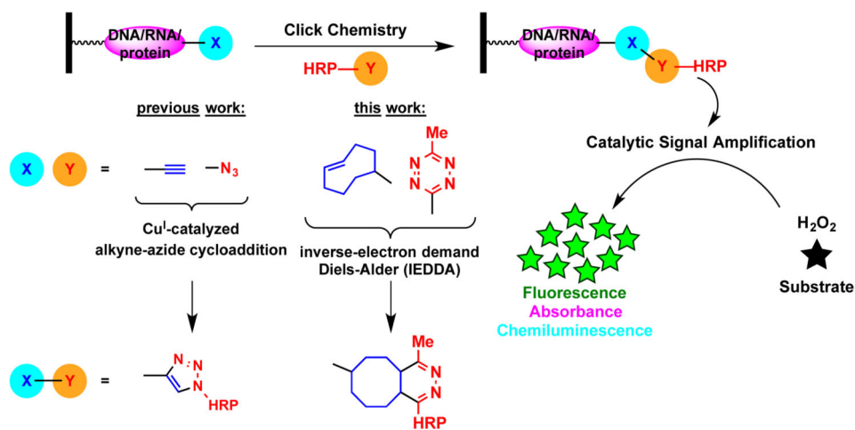
Fig. 1. cat-ELCCA scheme with modular click chemistry detection.
