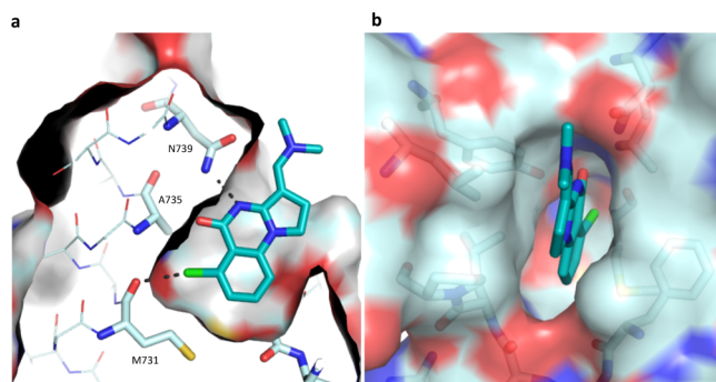
Figure 3. Cocrystal structure of 18 with PB1(5) at 1.5 Å (PDB code 5FH7): (a) cut-through illustrating positioning of chlorine in cavity; (b) surface view illustrating fit in PB1(5) pocket.
