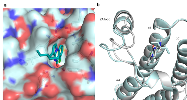
Figure 5. (a) Cocrystal structure of 28 with PB1(5) at 1.6 Å (PDB code 5FH8). (b) Overlay of PDB code 5FH7 (gray) of 18 and PDB code 5FH8 (cyan) of 28 showing the shift in the ZA loop of the PB1(5) domain on binding of 28 .
