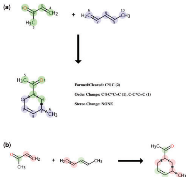
Fig. 1 (a) AAM performed by RDT and the resulting BCs (i.e. formed/cleaved: C%C (Ring), Order Change: C%*C=C (1), C-C*C=C (1) and (b) reaction centres are highlighted in pink colour in the image, where as neighbouring atoms are highlighted in green
