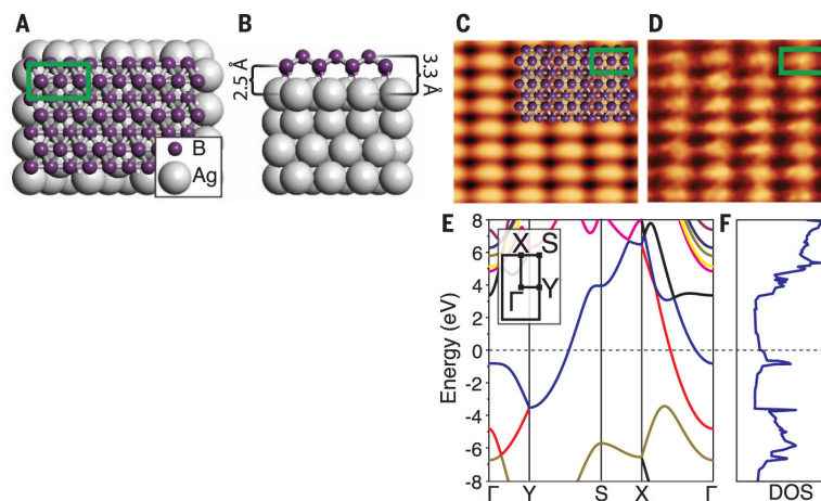
Fig. 2. Computational prediction of borophene structure and electronic properties
