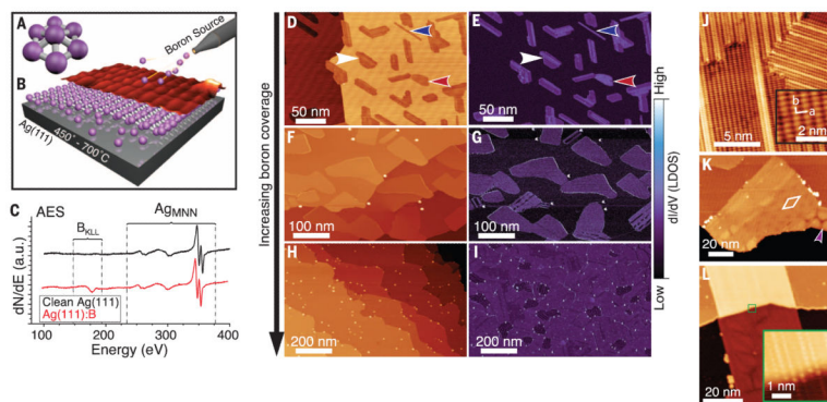
Fig. 1. Growth and atomic-scale characterization of borophene sheets
