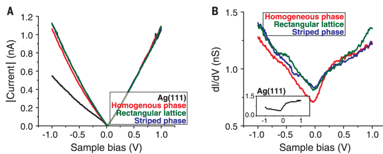
Fig. 4. Scanning tunneling spectroscopy of borophene
