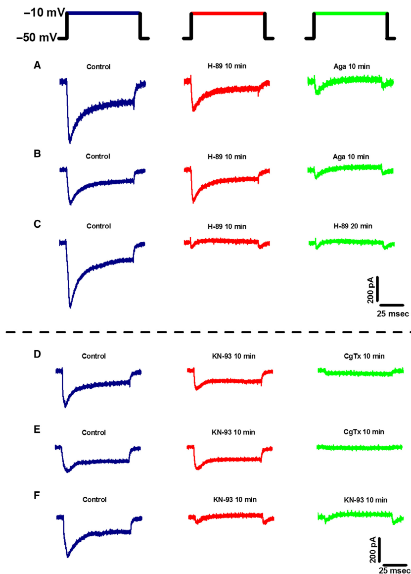
Figure 3. \text{Ca}^{2+} current ( I_{\text{Ca}} ) recordings illustrating the effects of H89 and KN-93 on PPN cells. All I_{\text{Ca}} were recorded using a multiple step depolarization protocol starting at -50 mV with 10 mV steps, up to 0 mV (top), but this figure shows only the -10 mV step. (A) I_{\text{Ca}} recorded from a PPN neuron (probably N + P/Q-type) before (navy), after 10 min of H89 (red record, reduction), and 10 min of CgTx (green, block). (B) I_{\text{Ca}} from a PPN neuron (probably P/Q-type) before (navy record), after 10 min of H89 (red, no effect), and 10 min of Aga (green record, block). (C) I_{\text{Ca}} recorded from a PPN neuron (probably N-type) before (navy), after 10 min of H89 (red, block), and 20 min of H89 (green, block). (D) I_{\text{Ca}} recorded from a PPN neuron (probably N + P/Q-type) before (navy record), after 10 min of KN-93 (red, reduction), and 10 min of CgTx (green, block). (E) I_{\text{Ca}} from a PPN neuron (probably N-type) before (navy), after 10 min of KN-93 (red record, no effect), and 10 min of CgTx (green, block). (F) I_{\text{Ca}} recorded from a PPN neuron (probably P/Q-type) before (navy), after 10 min of KN-93 (red record, block), and 20 min of KN-93 (green, block).
