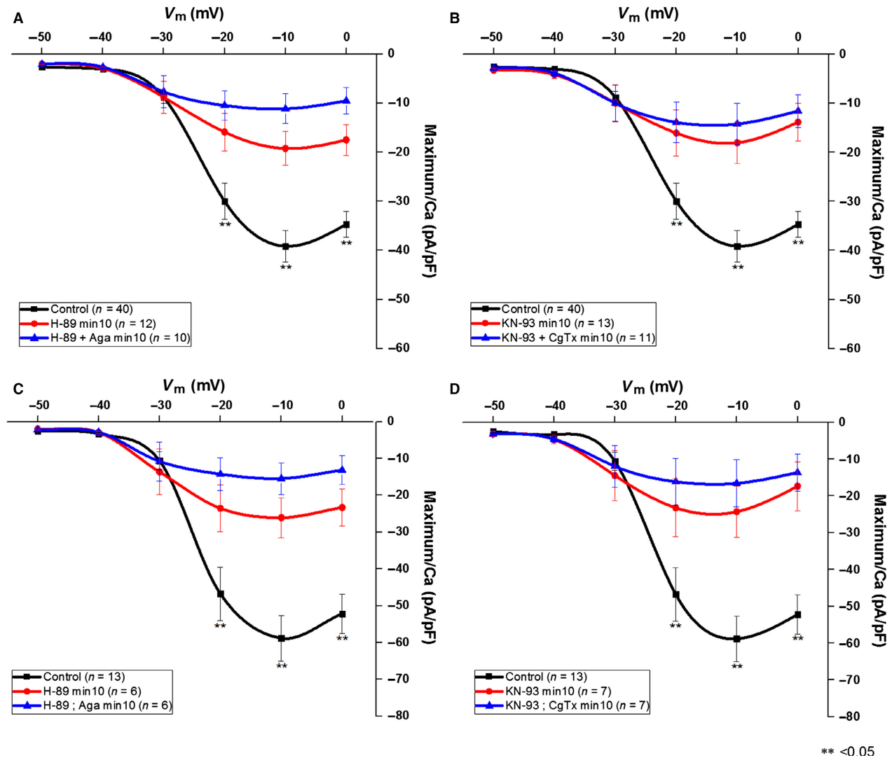
Figure 4. Average current-voltage ( I-V ) curve of I_{Ca} from PPN neurons. Note that high-threshold I_{Ca} peaked at \sim -10 mV. (A) Representative I_{Ca} current-voltage plot from all PPN control neurons ( n = 40 ) before treatment (black line). Red line shows maximum I_{Ca} (pA/pF) at min 10 for all PPN neurons ( n = 12 ) that were exposed to H89. Blue line shows maximum I_{Ca} (pA/pF) for all PPN neurons ( n = 10 ) that were exposed to H89 and Aga. (B) Representative I_{Ca} from all PPN control neurons ( n = 40 ) before treatment (black line). Red line shows maximum I_{Ca} (pA/pF) at min 10 for all PPN neurons ( n = 13 ) that were exposed to KN-93. Blue line shows maximum I_{Ca} (pA/pF) for all PPN neurons ( n = 11 ) that were exposed to KN-93 and CgTx. (C) I_{Ca} recordings from a population of PPN neurons ( n = 6 ) that were exposed to H89 and Aga sequentially. The black line represents the control condition. The red line represents I_{Ca} recordings after 10 min of H89. The blue line represents I_{Ca} recordings from neurons after 10 min of H89 and Aga. (D) I_{Ca} recordings from a population of PPN neurons ( n = 7 ) that were exposed to KN-93 and CgTx sequentially. The black line represents the control condition. The red line represents I_{Ca} recordings after 10 min of H89. The blue line represents I_{Ca} recordings from neurons after 10 min of H89 and Aga.
