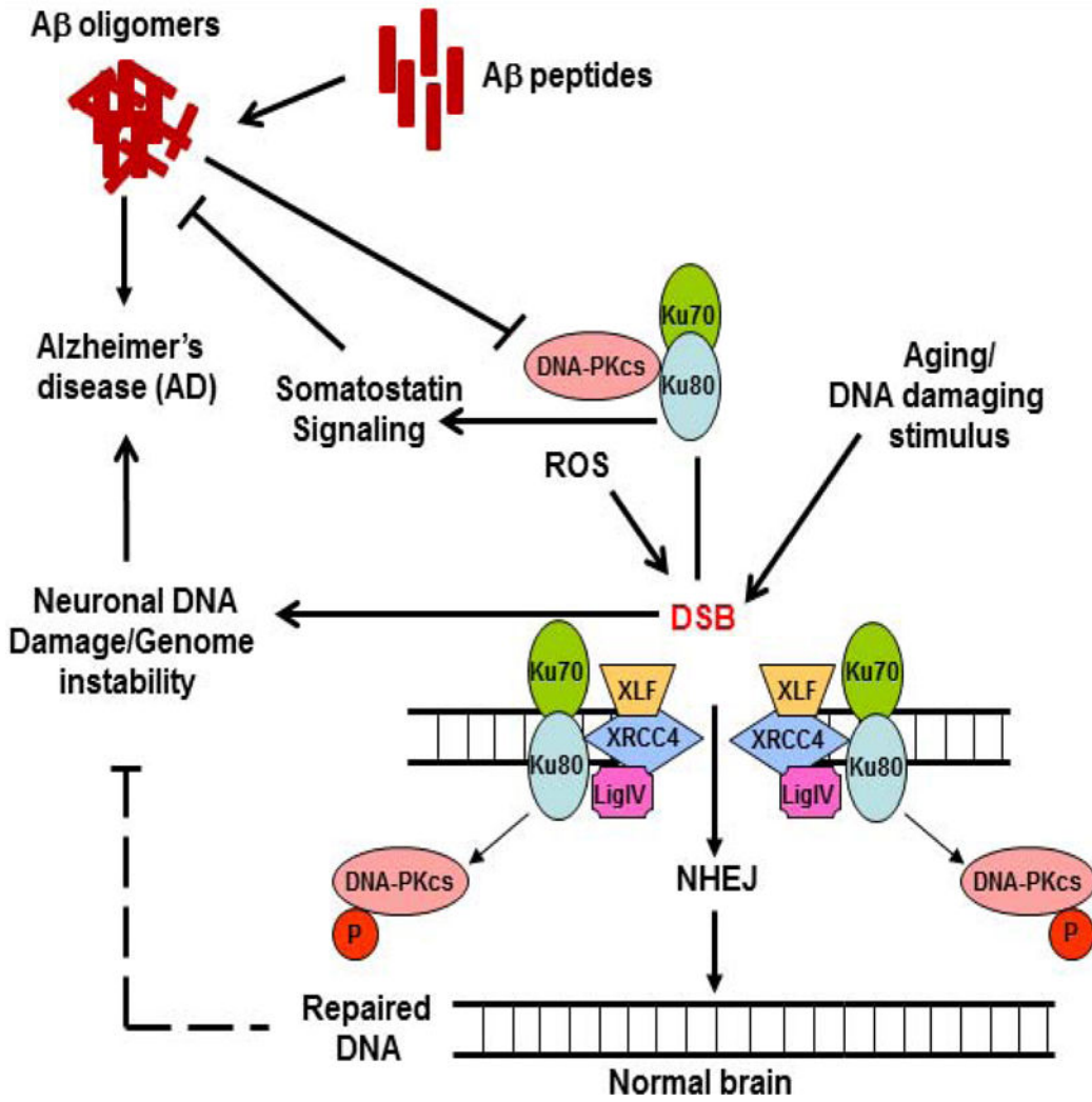
Figure 1. Schematic presentation of a potential link of DSB, DNA-PK and Aβ in AD brains. Upon induction of DSB either by normal aging/ROS or other DNA damaging agents, Ku80/Ku70 and DNA-PKcs are rapidly recruited to DNA ends, and DNA repair occurs as it would in normal cases. However, in AD brains, in addition to formation of Aβ oligomers from Aβ peptides, sustained DSB in the genome would cause genome instability leading to the loss of normal neuronal activity. Additionally, with depleted Ku80, a somatostatin receptor, disruption of somatostatin signaling could potentially induce Aβ generation thus accelerating AD pathology. DSB: DNA double strand break; DNA-PK: DNA-dependent protein kinase; ROS: Reactive oxygen species; Aβ Amyloid beta
