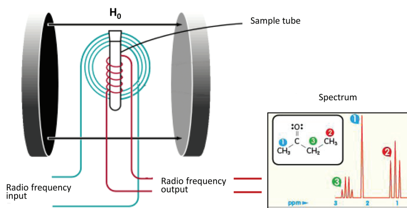
Figure 4. Principles of the proton nuclear magnetic resonance method for determining molecular structure.
