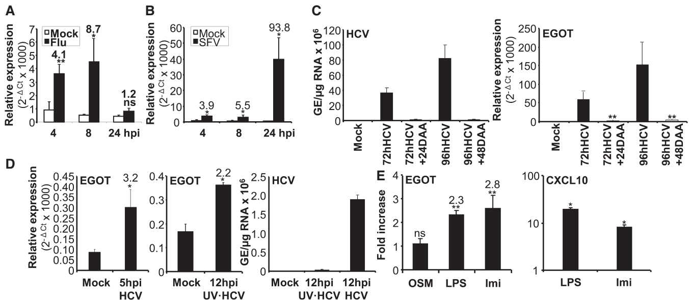
Figure 4. EGOT increases after infection with influenza, SFV or HCV and by TLR activation.
