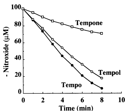
FIG. 4. Plot of the \cdot\text{O}_2^- -induced reduction rates of various piperidine nitroxides (100 \mu\text{M} ) in the presence of NADH (250 \mu\text{M} ). A reaction containing HX (2.5 mM) and XO (0.02 unit/ml) in air-saturated phosphate buffer (50 mM, pH 7.8) containing 50 \mu\text{M} DTPA and CAT (100 units/ml) was used to generate \cdot\text{O}_2^- . The rates of reduction were measured following the addition of XO by continually monitoring the EPR signal intensities of the nitroxides. Closed circles, Tempo; open circles, Tempol; and open squares, Tempone.
