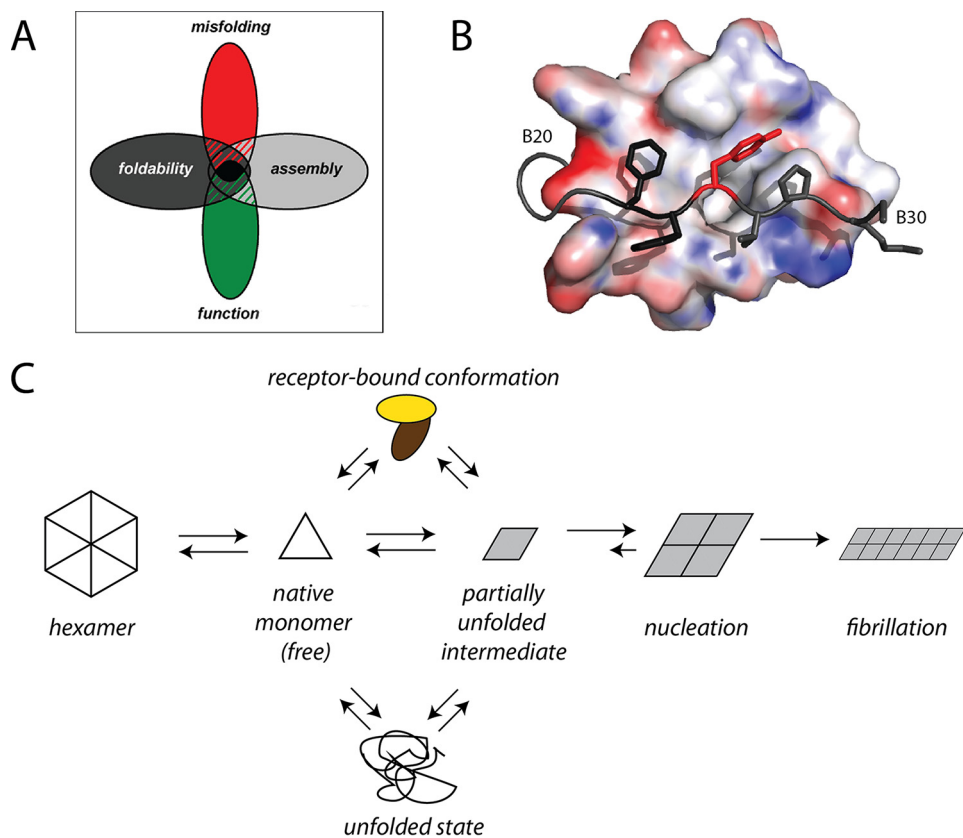
FIGURE 7. Evolutionary constraints and insulin fibrillation. A , Venn diagram showing intersection of multiple constraints: function, foldability, misfolding, and assembly. We envisage that Tyr B26 is conserved due to its explicit roles in folding and assembly and implicit role in avoiding misfolding. B , surface representation of a T-state monomer (PDB entry 4INS) with residues B23–30 (stick model) within a groove between the A and B chains. The aromatic side chains of Phe B24 and Phe B25 (both dark gray) and Tyr B26 (red) are shown. C , general scheme of insulin fibrillation via a partially unfolded monomer intermediate. The native state is protected by classic self-assembly. Disassembly leads to an equilibrium between native and partially folded monomers. The receptor-bound conformation of insulin (top) may also participate in this equilibrium. This partial fold may unfold completely (bottom) as an off-pathway event or aggregate to form a nucleus en route to a proto-filament (right).
