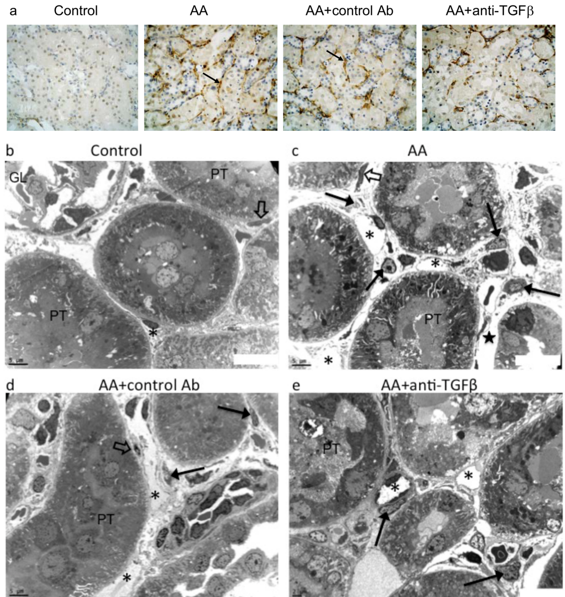
Fig 8. Representative photomicrographs of platelet-derived growth factor receptor beta (PDGFRβ) expression in the kidney tissues. (a) Absence of PDGFRβ staining in control rats and enhanced PDGFRβ expression detected around proximal tubules in the areas of medullary rays in kidney section in AA and AA+control Ab, but weak PDGFRβ staining was observed in the anti-TGFβ group. (b) In the control group, normal ultrastructure of kidney interstitium, resident fibroblast (open arrow) characterized by elongated nuclei firmly attached to the proximal tubules (PT), peritubular capillary (*). (c and d) In AA and AA+control Ab groups, increased number enlarged peritubular capillaries (*) with adjacent myofibroblasts (black arrows), obvious interstitial edema (★), (e) less severe peritubular capillary injury (*) with closely attached myofibroblasts (black arrows) (F). Original magnifications: (b-d) x2500 and (e) x3000.
