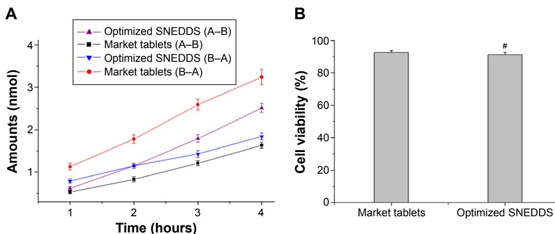
Figure 5 Transport amount of cyclovirobuxine D in 4 hours (A) and Caco-2 cell viability after transport study (B) ^{\#}P > 0.05 vs market tablets. Abbreviations: SNEDDS, self-nanoemulsifying drug delivery system; A–B, from apical side to basolateral side; B–A, from basolateral side to apical side.
