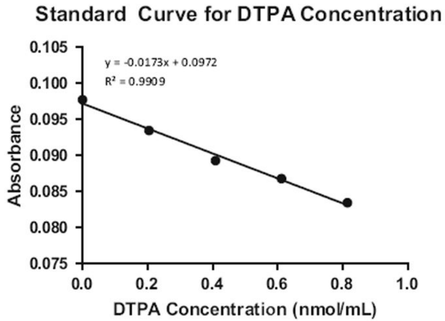
Fig. 1. Scatter plot obtained from creating the standard curve of the DTPA concentrations. As seen below, the final concentration of DTPA added to the cuvette is on the X -axis, and absorbance at 652 nm is on the Y -axis. From here, concentration of the DTPA inside the siRNA–DTPA mixture can be obtained
