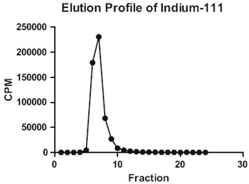
Fig. 2. Scatter plot obtained from purifying and eluting ^{111}\text{Indium} -labeled siRNA over a PD-10 column. The radioactivity as measured in counts per minute (CPM) are shown on the Y -axis as a function of the fraction eluted on the X -axis. A clear peak is shown in fraction 7
