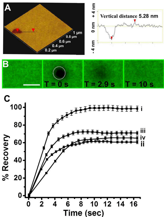
FIGURE 4 FRAP experiments in C-dot-DMPC/DOPC SSBs. (A) AFM image of an SSB (left) and the corresponding height profile (right). The size of the AFM image is 1 \mu m \times 1 \mu m. (B) Confocal fluorescence microscopy images (excitation at 405 nm, emission filter EM 445/60) recorded at different times after photobleaching by a 405 nm laser (time immediately after laser irradiation is defined as T = 0 s). The bleached region is indicated by the circle. Scale bar, 5 \mu m. (C) Recovery curves recorded upon incubation of the SSBs with different molecules: control SSB (i), PMB (ii), valproic acid (iii), and A \beta_{1-40} (iv). Each experiment was repeated five times. To see this figure in color, go online.
