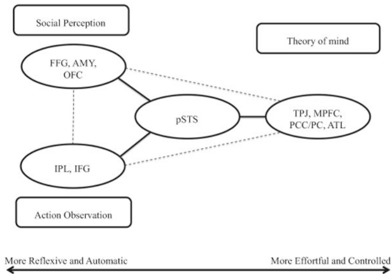
Fig. 1. An integrative model of the neural systems for social information processing: social perception, action observation, and theory of mind. Dashed lines suggest possible connections among these systems. AMY, amygdala; FFG, fusiform gyrus; OFC, orbitofrontal cortex; pSTS, posterior superior temporal sulcus; IFG, inferior frontal gyrus; IPL, inferior parietal lobule; MPFC, medial prefrontal cortex; TPJ, temporo-parietal junction; PCC/PC, posterior cingulate cortex/precuneus; ATL, anterior temporal lobe.
