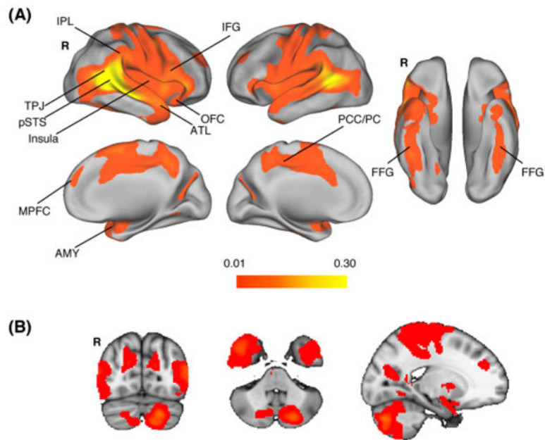
Fig. 3. Resting-state functional connectivity with a sample of 1000 subjects and a seed voxel in the pSTS at (52, -46, 9), MNI152mm coordinate, i.e., the center of gravity in Fig. 2(D). The result was the average of the results based on seed voxels at (52, -46, 10) and (52, -46, 8) and the maps were available from the Neurosynth website. The strength of functional connectivity is based on correlations, with higher values indicating greater similarity in activation between the seed voxel in the pSTS and other voxels of the brain. For details of these maps, see Yeo et al. (2011), Buckner et al. (2011), and Choi et al. (2012). Top Panel (A) shows that the pSTS is functionally connected to the major regions implicated in social information processing (see the integrated model in Fig. 1). Bottom Panel (B) shows functional connectivity from the seed voxel in the pSTS to cerebellar cortex. The slice was at (-19, -76, -41), MNI152mm coordinate.
