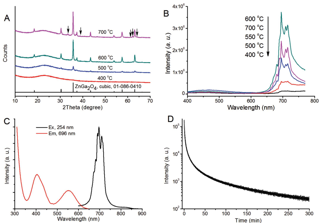
Figure 1. Optimization of the experimental conditions. A) XRD and B) photoluminescence spectra (excitation wavelength, 254 nm) of the mZGC samples synthesized at various temperatures, C) PL excitation and emission spectra (tested by using the phosphorescence mode of the fluorimeter), D) PL decay curve of mZGC synthesized at 600 °C, excited by UV lamp (254 nm). Sample mass for above measurements are 100 mg.
