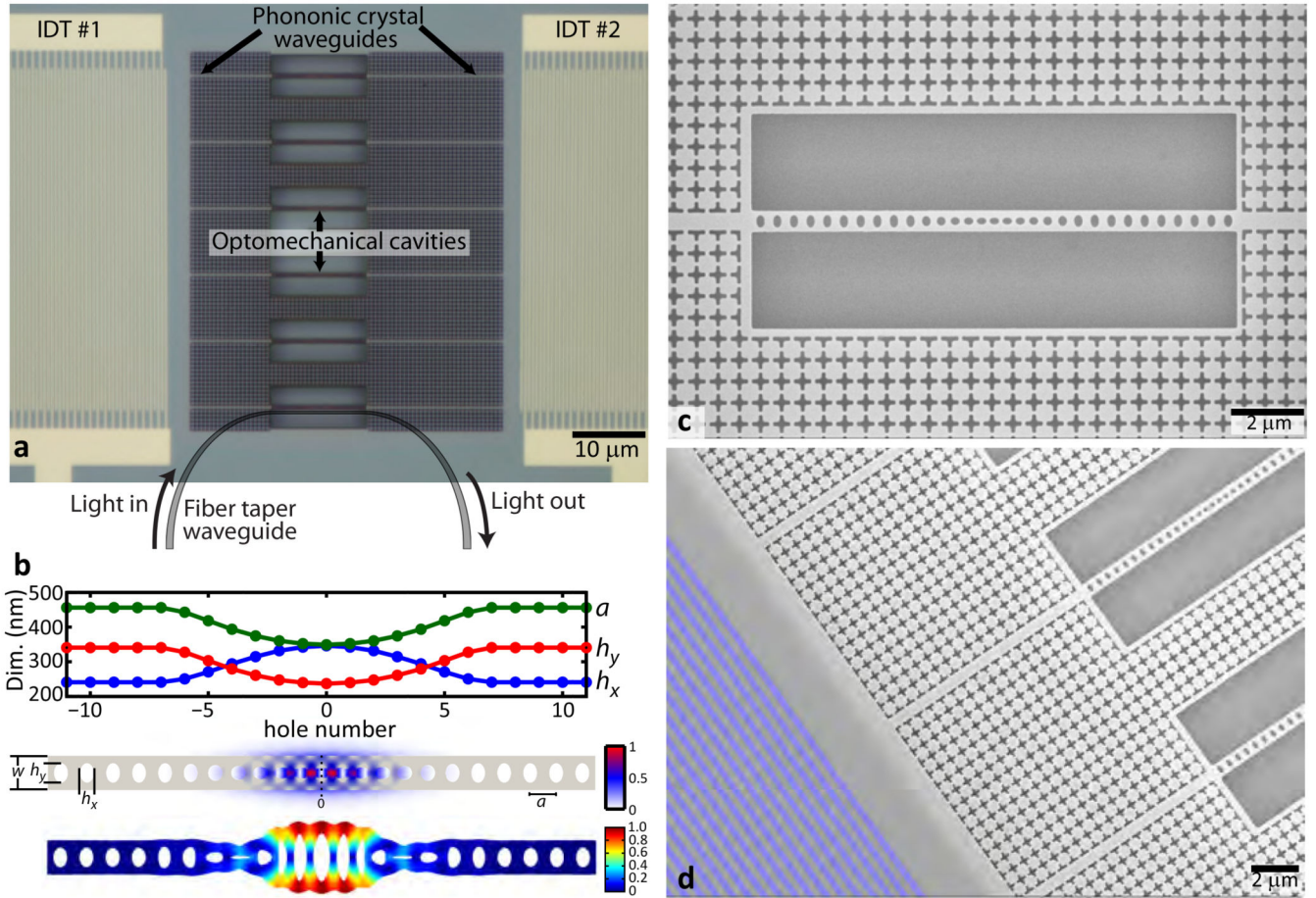
FIG. 1. Piezo-optomechanical circuits
