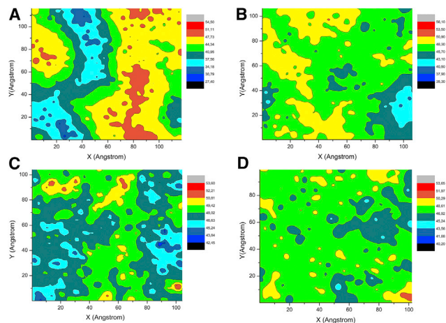
FIGURE 9 (a–d) Projection of a thickness profile in the xy plane of a phospholipid bilayer containing a 1:2 molar ratio of DOPC/DPPC, averaged after 150 ns of atomistic MD simulations with the following contents of cholesterol: (a) 0%, (b) 20%, (c) 30%, and (d) 40%. The thickness profile was evaluated by considering the average phosphorus-to-phosphorus distance. To see this figure in color, go online.
