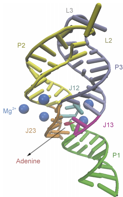
FIG. 1. Three-dimensional structure of add A-riboswitch with five Mg^{2+} ions and a ligand adenine (PDB code 1Y26). The ligand and Mg^{2+} ions are colored with red and blue, respectively. The secondary structures of the system are labelled correspondingly with P1, P2, and P3 for stems, L2 and L3 for loops, and J12, J13, and J23 for junctions.
