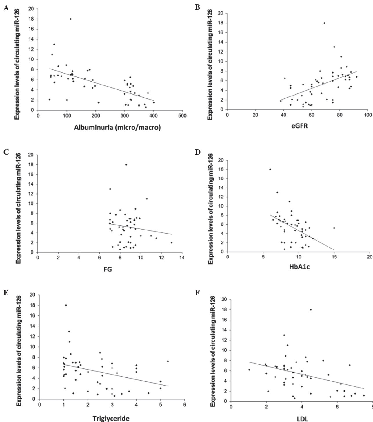
Figure 3. Correlation between circulating miR-126 and renal function parameters and other clinical variables. Pearson's coefficient correlation analysis was undertaken in patients with DN to determine the correlation between circulating miR-126 levels and albuminuria, eGFR, FG, HbA1c, triglyceride and LDL. (A) Circulating miR-126 negatively correlated with albuminuria. (B) Circulating miR-126 positively correlated with eGFR. (C) Circulating miR-126 negatively correlated with FG. (D) Circulating miR-126 negatively correlated with HbA1c. (E) Circulating miR-126 negatively correlated with triglyceride. (F) Circulating miR-126 negatively correlated with LDL.
