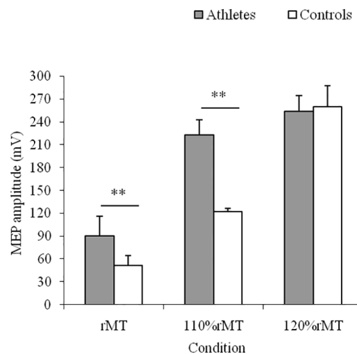
Fig 2. Motor Evoked Potential (MEP) Amplitude. Means and SDs of MEP amplitude in the three experimental conditions for karate athletes and controls.
