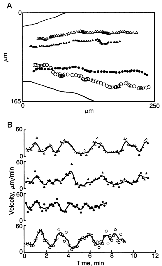
FIG. 2. Periodic cell movement in the prespore zone shown in Fig. 1E. (A) Tracks of four anterior-like cells. Solid lines show the position of the slug at the beginning of the measurement. The slug moves from left to right. (B) Velocity changes of these same cells. The solid line is derived from the data points by moving average smoothing over three neighboring points. Symbols in B correspond to symbols in A.
