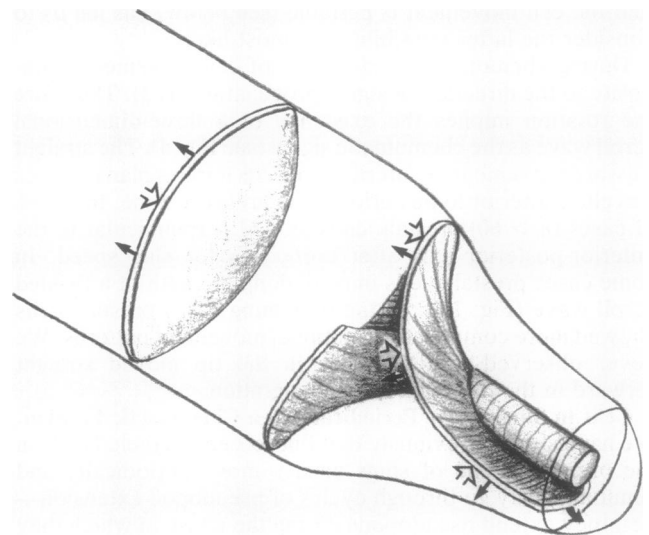
FIG. 4. Model of signal propagation and cell movement in slugs. The observed cell movement is explained by chemotaxis to a scroll wave propagating in the prestalk zone, which unwinds to planar waves in the prespore zone. The intersection of the wave front with the visible surface of the slug is shown as a double line. Black arrows indicate the direction of signal propagation. Open arrows indicate the direction of cell movement. The direction of cell movement is opposite to the direction of signal propagation. The scroll wave in the tip rotates around a central core, in which the cells are adapted. The exact nature of the transition of the scroll wave in the tip to planar waves in the prespore zone is unknown. However, for better visualization we have drawn an imaginary transition. The strong curvature of the wave front at the prestalk/prespore boundary is in agreement with the observed cell movement. Understanding the exact nature of the transition (what happens in the core) will be crucial to complete understanding of three-dimensional wave propagation. This will require detailed mathematical modeling and further experimentation.
