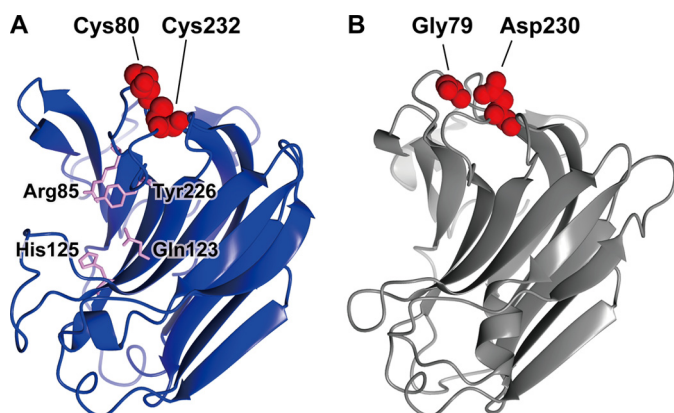
FIGURE 8. Homology modeling of NitAly and PyAly. The structures of NitAly ( A , residues 34–242) and PyAly ( B , residues 13–216) were predicted using the PHYRE2 program (63) and P. aeruginosa alginate lyase PA1167 (Protein Data Bank code 1vav) as the template (15) with 100% confidence, respectively. A , Cys-80 and Cys-232 are shown by red globules. The residues Arg-85, Gln-123, His-125, and Tyr-226, which correspond to the suggested catalytic residues in PA1167 (15, 21), are shown by pink sticks. B , Gly-79 and Asp-230 are shown by red globules.
