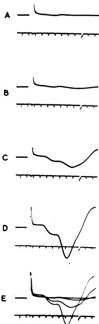
FIG. 5. Effect of increasing intensity of stimulation (a-d). In (e) each is superimposed. Time scale in milliseconds.
