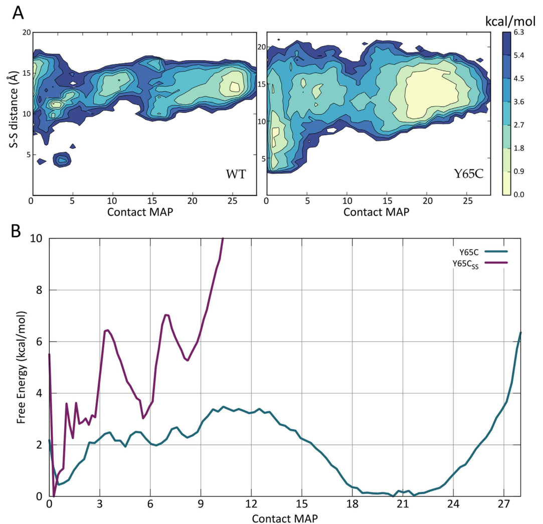
Figure 4. (A) Reweight of the Free Energy along the distance between the sulfur atoms of residues Cys60 and Cys65 (Tyr65 in the WT). The population of structures with a low distance between the two residues is increased in the Y65C mutant, with values as low as 4 Å in the unfolded state (CMAP < 5) of both proteins. (B) Free Energy of the Y65C mutant with and without the disulphide bridge between Cys60 and Cys65 as a function of the contact map.
