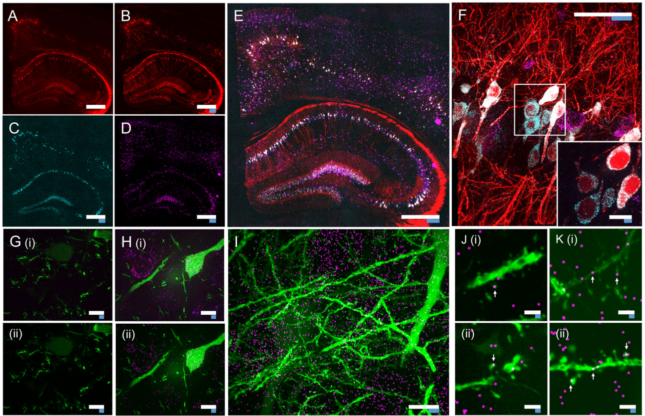
Figure 3. Nanoscale imaging of RNA in mammalian brain. (a) Widefield fluorescence image of Thy1-YFP mouse brain. (b) Post-expansion widefield image of (a) . (c) Widefield fluorescence showing HCR-ExFISH of YFP mRNA in the sample of (b) . (d) As in (c) , but for Gad1 mRNA. (e) Composite of (b-d) , highlighting distribution of Gad1 versus Thy1-YFP mRNAs. (f) Confocal image of mouse hippocampal tissue from (e) showing single RNA puncta. Inset, one plane of the boxed region (red, YFP protein; cyan, YFP mRNA; magenta, Gad1 mRNA). (g) Confocal image (i) and processed image (ii) of HCR-ExFISH using a missense Dlg4 probe, in Thy1-YFP mouse tissue (green, YFP protein). The raw image (i) uses alternating probes in two colors (red, Dlg4 missense even; blue, Dlg4 missense odd). The processed image (ii) shows zero co-localized spots (magenta). (h) As in (g) , but for HCR-ExFISH targeting Actb in Thy1-YFP mouse brain (green, YFP protein; red, Actb even, and blue, Actb odd in (i) ; co-localized spots in magenta (ii) ). (i) Confocal image of hippocampal tissue showing co-localized Dlg4 puncta (magenta) overlaid on YFP (green). (j) Dendrites with Dlg4 mRNA localized to spines (arrows). (i) , (ii) , two representative examples. (k) As in (j) , but with HCR-ExFISH of Camk2a mRNA showing transcripts in dendritic spines and processes. Scale bars (white, in pre-expansion units; blue scale bars are divided by the expansion factor noted): (a) 500 \mu\text{m} ; (b-e) 500 \mu\text{m} (expansion factor 2.9 \times ); (f) 50 \mu\text{m} (2.9 \times ), inset 10 \mu\text{m} ; (g-i) 10 \mu\text{m} (3 \times ); (j,k) 2 \mu\text{m} (3 \times ). (e,i) maximum-intensity projection (MIP) 27 \mu\text{m} thick (pre-expanded units); (g,h,j,k) MIPs ~1.6 \mu\text{m} thick.
