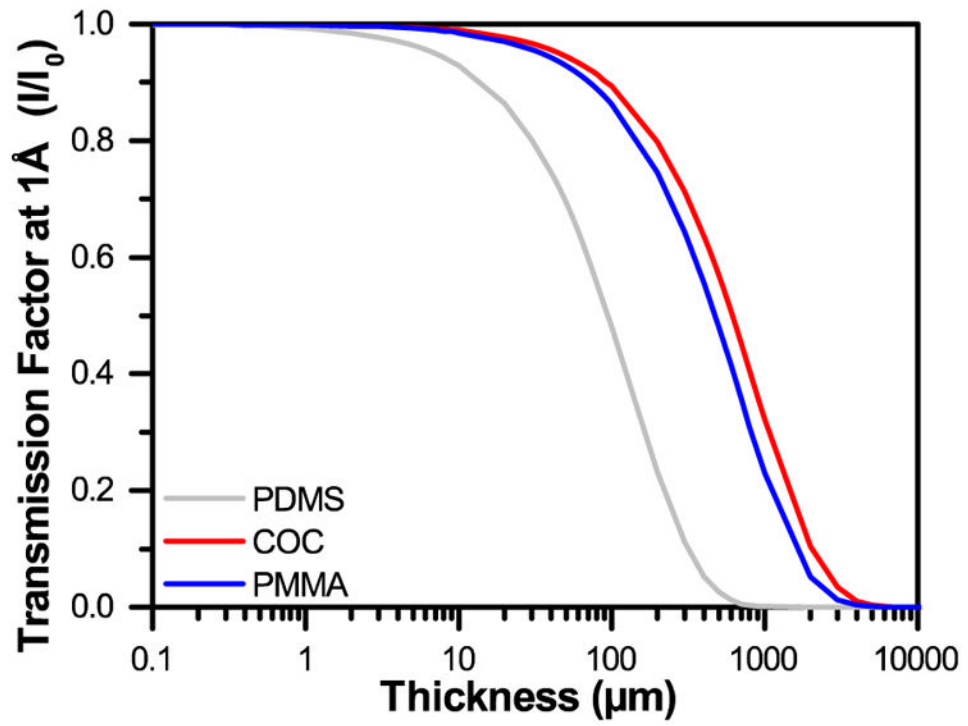
Fig. 1. A comparison of the transmission factors I/I_0 for varying thicknesses of PDMS, COC, and PMMA at an X-ray energy of 12.4 keV, or a wavelength of 1Å.
