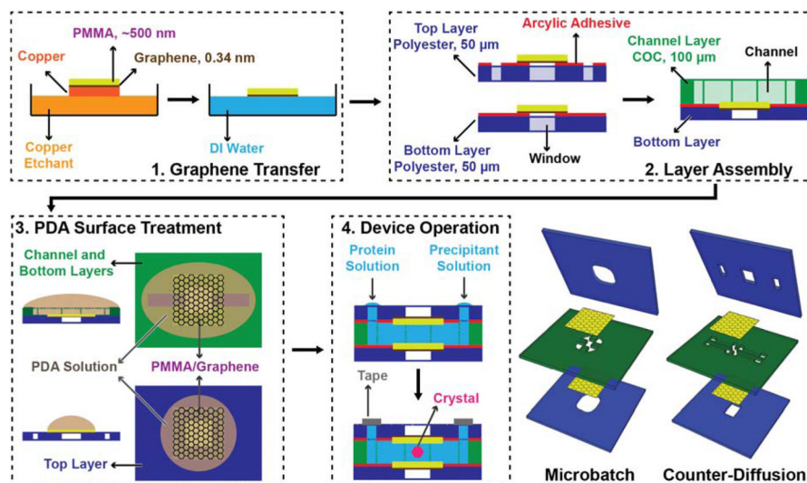
Fig. 2. Schematic depiction of the fabrication scheme for thin-film graphene-based microfluidics, using a channel-based counter-diffusion as the example. (1) CVD-grown graphene on copper is first coated with a layer of PMMA, and then released from the copper substrate by etching. The subsequent film is floated on the surface of water for (2) transfer to an adhesive polyester support layer to define the window areas of the device. This layer is then adhered to a COC layer containing the cut-out pattern for the microfluidic channels. (3) A hydrophilic PDA surface treatment on both the top PMMA/graphene film and the bottom layer containing the microfluidic channel facilitates easy filling of the final device via capillary action. (4) The final, assembled device is held together by the adhesive layers defining the window structures, leaving the PMMA/graphene window areas free of excess material. Either microbatch or counter-diffusion crystallization trials can be set up by the addition of protein and precipitant solutions. The device inlets are sealed with Crystal Clear tape.
