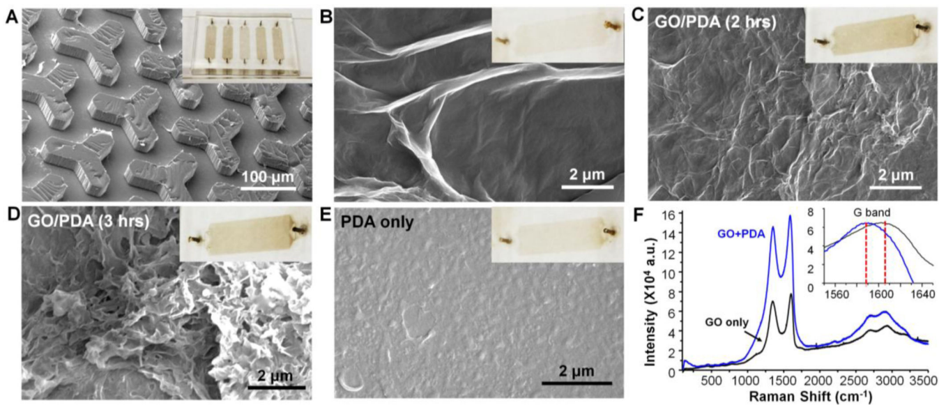
Figure 2. Characterization of microfluidic GO/PDA coating. (A) SEM image and digital image (inset) of a GO/PDA-coated chip containing the Y-shaped PDMS microposts. (B) SEM image of a GO-coated channel (inset) showing the microscale 3D surface topology formed by GO coating. (C, D) SEM of the GO/PDA-coated channels with different reaction time for PDA deposition (inset) showing distinct morphologies of the GO/PDA interface. (E) SEM image of the PDA-coated channel (inset) showing a much smoother and more solid PDA film formed on the surface without GO coating. (F) Raman spectra of the coatings. Inset: red shift of the G band of GO after PDA coating. The GO/PDA plot is offset for comparison.
