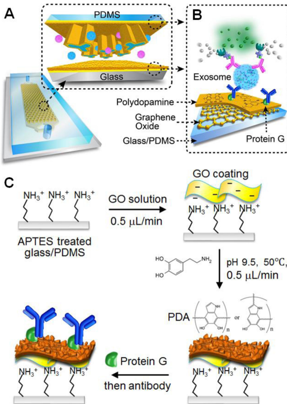
Figure 1. The nano-interfaced microfluidic exosome platform (nano-IMEX). (A) Schematic of a single-channel PDMS/glass device, with the exploded-view highlighting the coated PDMS chip containing an array of Y-shaped microposts. (B) Surface of the channel and microposts coated with graphene oxide (GO) and polydopamine (PDA) as a nanostructured interface for the sandwich ELISA of exosomes with enzymatic fluorescence signal amplification. (C) The procedure for surface functionalization of the microfluidic chips.
