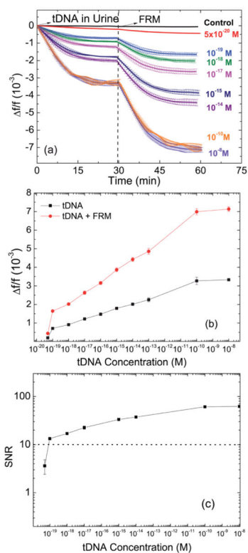
Fig. 8. (a) Relative resonance frequency shift \Delta f/f versus time of tDNA detection at various concentrations in urine and (b) – \Delta f/f at t = 30 min (tDNA hybridization) and at t = 60 min (tDNA hybridization plus FRM detection) versus tDNA concentration. (c) SNR versus concentration of tDNA graph plotted using data in (a).
