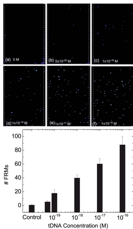
Fig. 9. Fluorescent micrographs of the PEPS surface after FRM detection followed by (a) 0 M, (b) 5 \times 10^{-20} M, (c) 1 \times 10^{-19} M, (d) 1 \times 10^{-18} M, (e) 1 \times 10^{-17} M and (f) 1 \times 10^{-16} M of tDNA detection. The width of PEPS B as denoted by the parallel dashed lines was 450 \mu\text{m} . Clearly, the number of FRMs captured on the PEPS surface increased with an increasing tDNA concentration in a dose responsive fashion validating the tDNA detection at a concentration as low as 5 \times 10^{-20} M. (g) Average number of FRMs captured on the PEPS surface versus tDNA concentration in urine.
