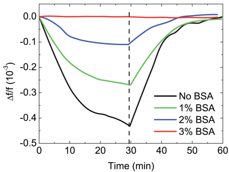
Fig. 7. Relative frequency shift, \Delta f/f , of PEPS B in urine at 1 \text{ ml min}^{-1} for 30 min followed by PBS washing at a flow rate of 6 \text{ ml min}^{-1} after the PEPS was initially blocked with 0, 1, 2 and 3 % BSA.
