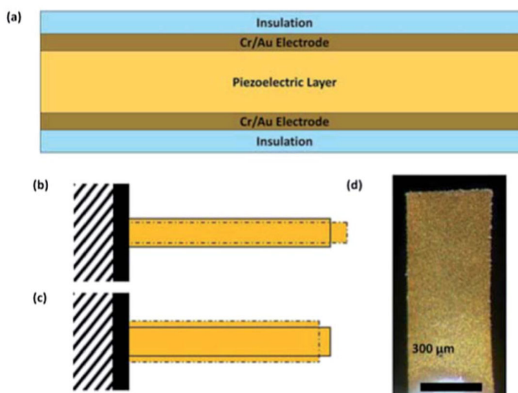
Fig. 1. A schematic of (a) the cross-section of a piezoelectric plate sensor (PEPS), (b) the first length extension mode (LEM), (c) width extension mode (WEM) vibration of a PEPS where the solid bars illustrate the initial position of the PEPS and the dashdotted shapes illustrate the extended positions, and (d) a top-view optical micrograph.
