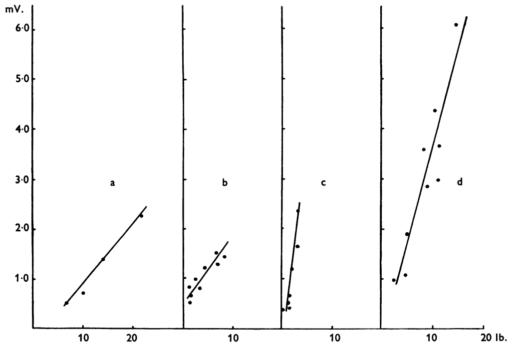
FIG. 5.—Voltage tension curves from triceps of a healthy subject and three patients with muscular weakness. (a) Healthy subject, b = 0.1386 ; (b) Case 22, motor neurone disease, b = 0.1292 ; (c) Case 23, muscular dystrophy, b = 0.9798 ; (d) Case 24, poliomyelitis, b = 0.3809 .
