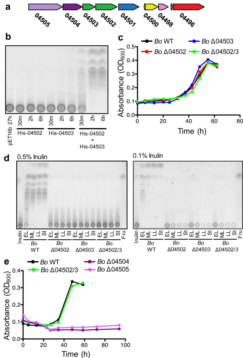
Figure 2. B. ovatus does not require surface digestion for utilization of inulin a , Predicted inulin utilization locus of B. ovatus ( Bo ). Gene designations shown are preceded by BACOVA_. The color coding of gene products is as in Fig.1. b , Thin layer chromatography (TLC) analysis of inulin defined medium incubated for the indicated times with purified His-tagged 04502, 04503 or 04502 and 04503, or vector control. See SI Figure 1 for uncropped scanned images. c , Growth of Bo WT and mutants in inulin defined medium. d , TLC analysis of conditioned media during the growth of Bo WT and mutants in 0.5% and 0.1% inulin. EL = early log, ML = mid log, LL = late log, St = stationary. e , Growth of Bo WT, 04502/3, 04504 ( susD ortholog) and 04505 ( susC ortholog) mutants in inulin defined medium. For c,e , each line represents n=1 sample per condition. See Extended Data Fig.2 for additional independent experiments. In all panels error bars represent standard error; p values derived from two-tailed Student's t test.
