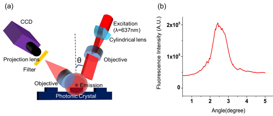
Figure 4. (a) Schematic diagram of the detection instrumentation. (b) Fluorescence intensities obtained from 50µg/mL LD700 solution filled within the channel when excited over a range of illumination angles.
