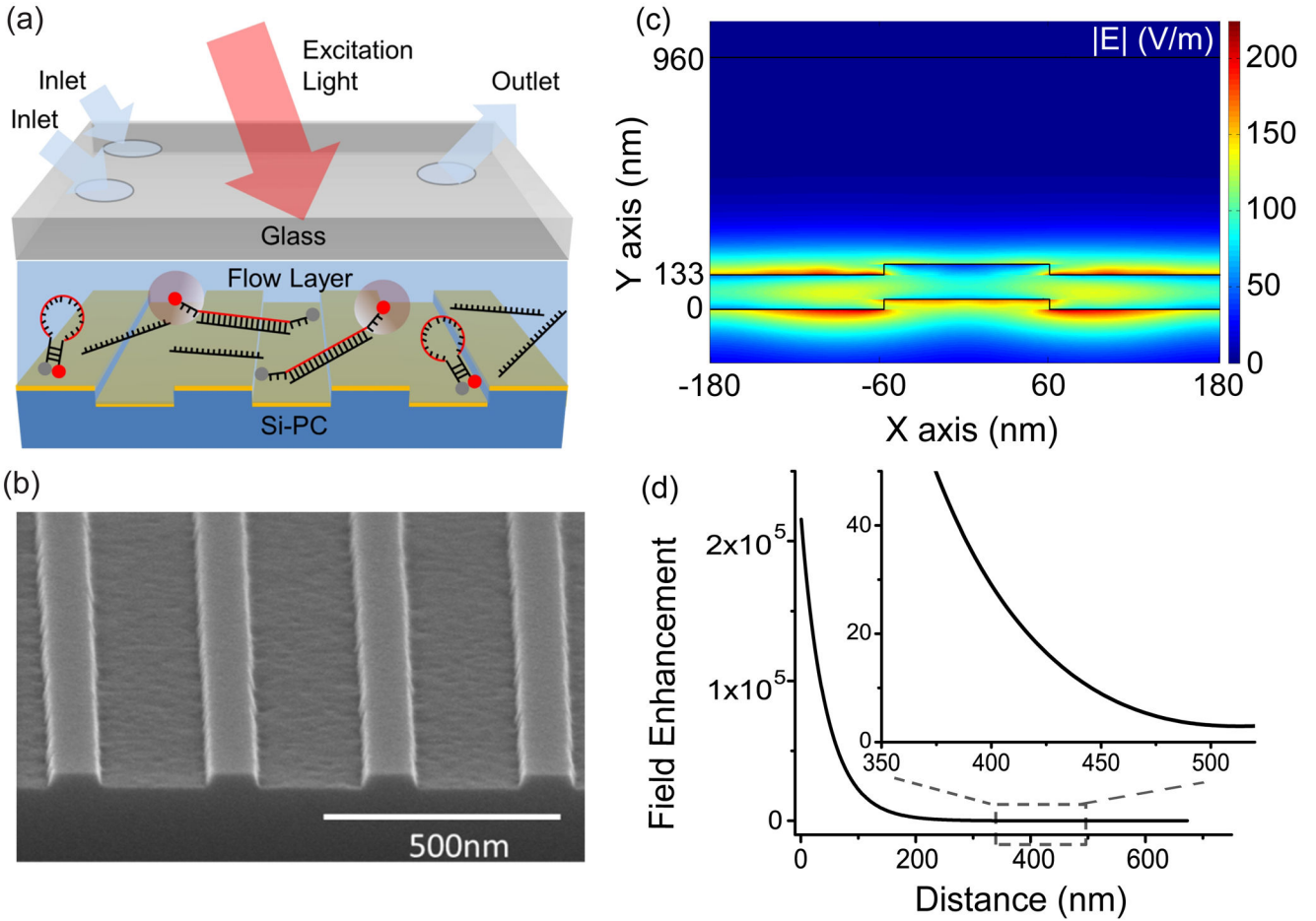
Figure 1. (a) Schematic diagram of the device structure, comprised of a transparent glass layer, a microfluidic region and a PC surface for fluorescence enhancement. (b) SEM image of the one dimensional PC with period of 360nm and duty cycle of 36%. (c) Evanescent electric field enhancement distribution at the resonant coupling condition of the PC (d) The average enhancement of field intensity as the function of distance, d , above the top \text{TiO}_2 layer of the PC.
